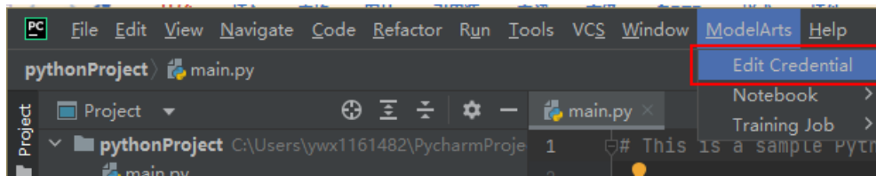
图 6-83 Edit Credential
