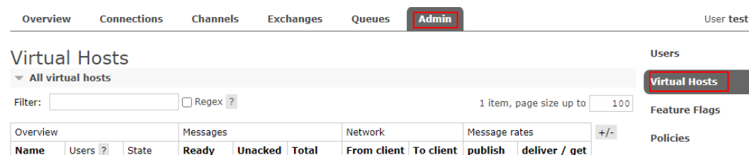
图 4-4 Virtual Hosts
