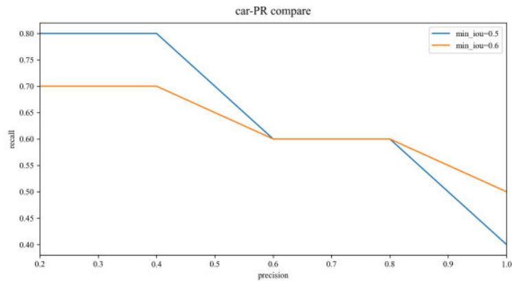
图 6-4 car-PR compare
