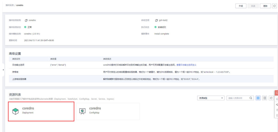
图 11-5 CoreDNS Deployment
