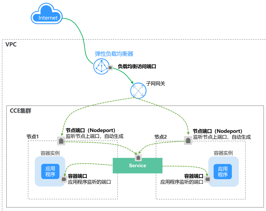
图 3-151 负载均衡 (LoadBalancer)
