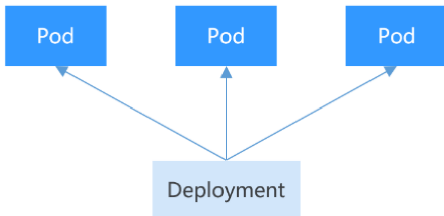
图 3-77 Deployment
