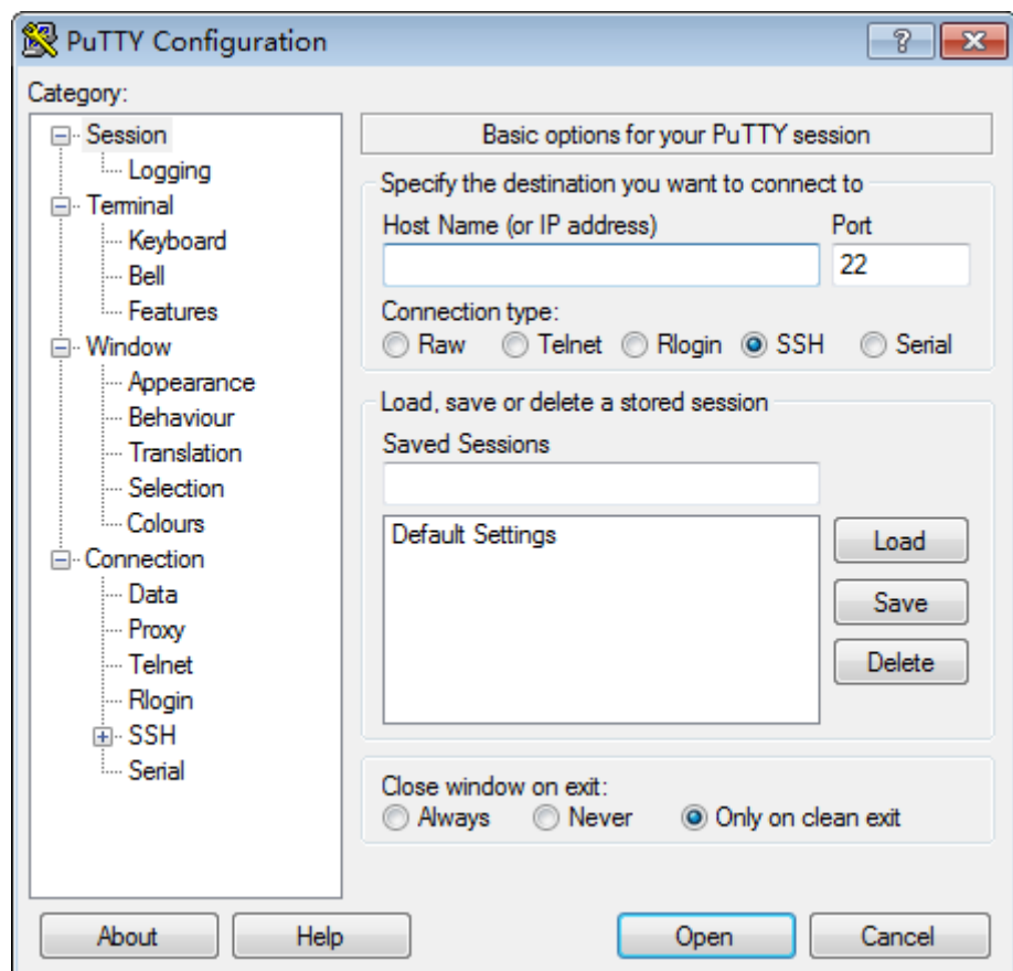
图 2-7 PuTTY Configuration
