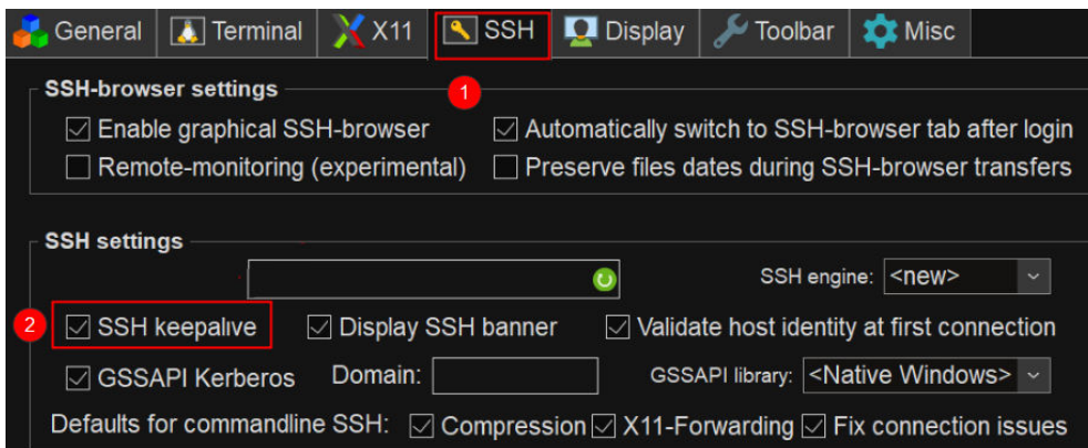
图 5-35 勾选“SSH keepalive”
