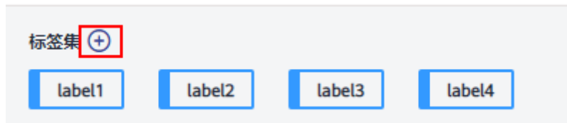
图 7-35 添加标签 (1)
