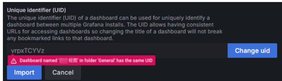
图 11-14 修改 uid
