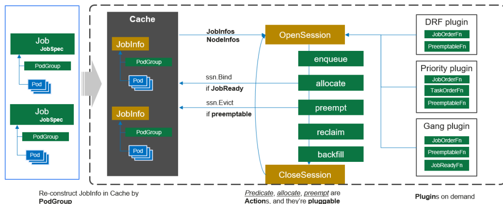
图 3-105 Volcano Scheduler workflow
