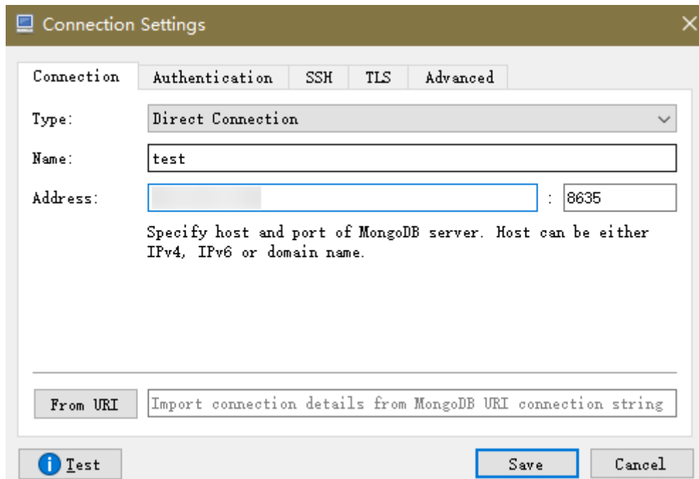
图 2-40 Connection
