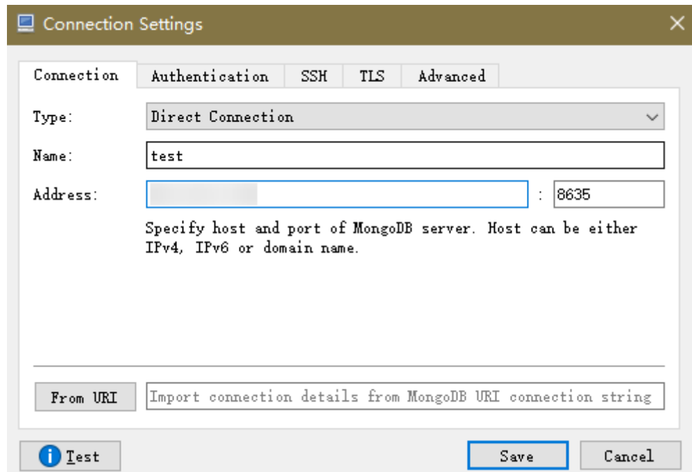
图 3-38 Connection
