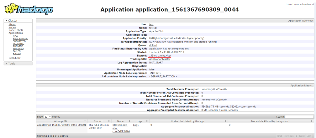
图 6-7 application
