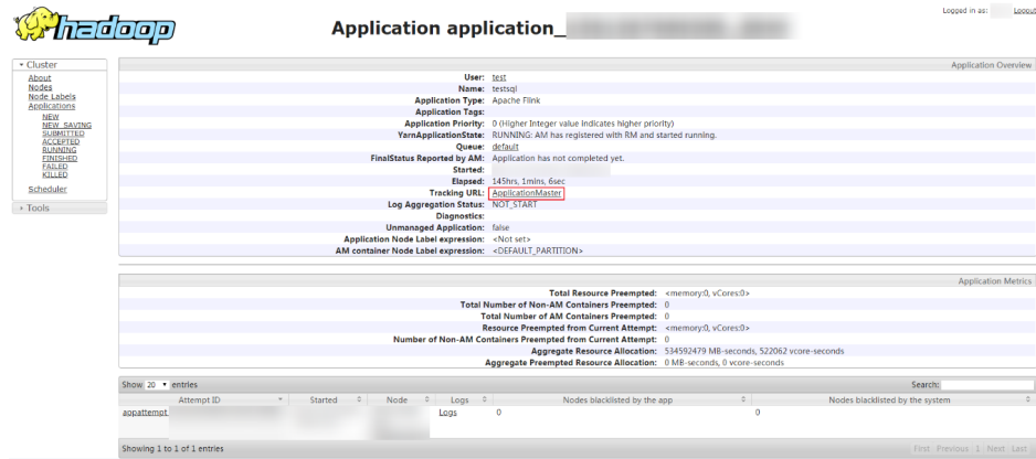
图 12-11 application
