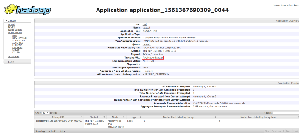
图 6-11 application
