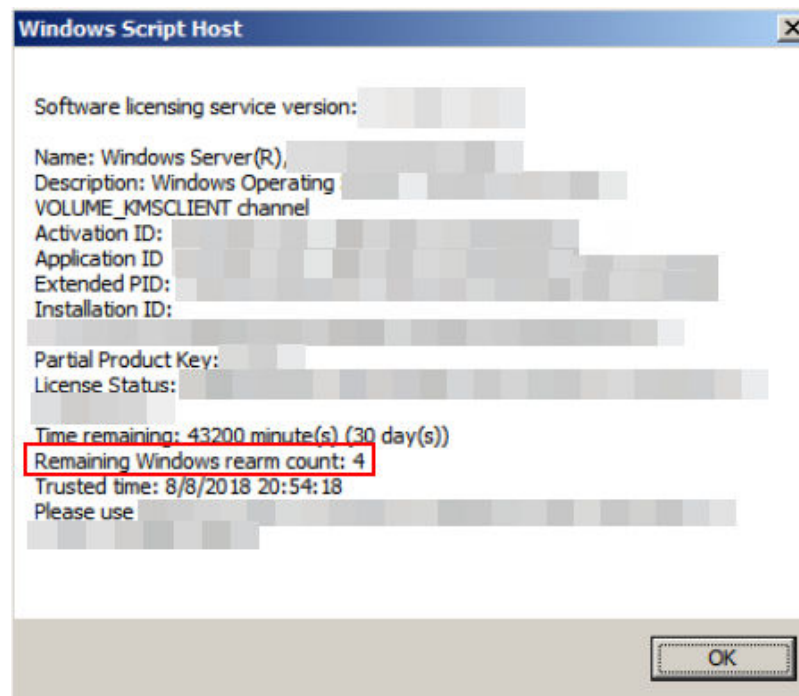
图 4-7 Windows Script Host
