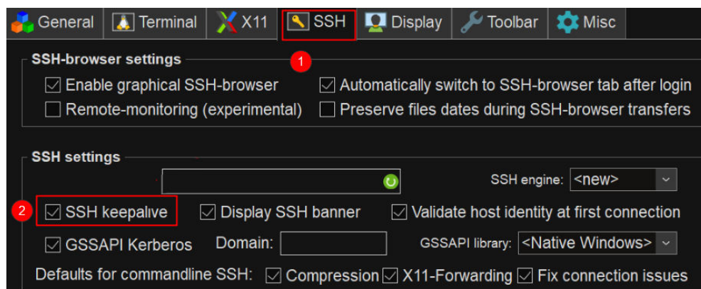
图 5-20 勾选“SSH keepalive”
