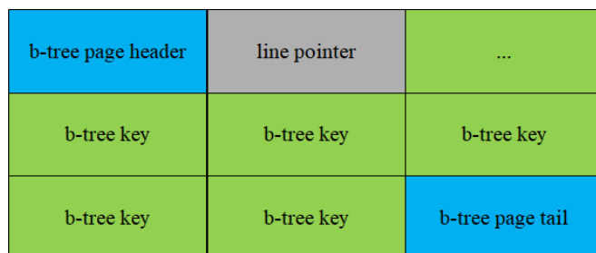
b-tree key
