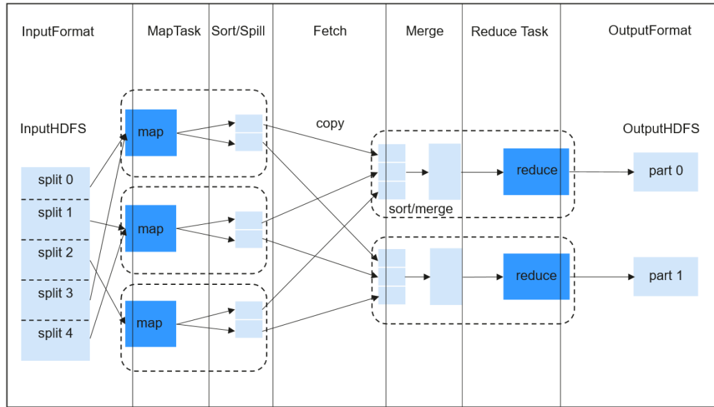
图 1-77 MapReduce job
