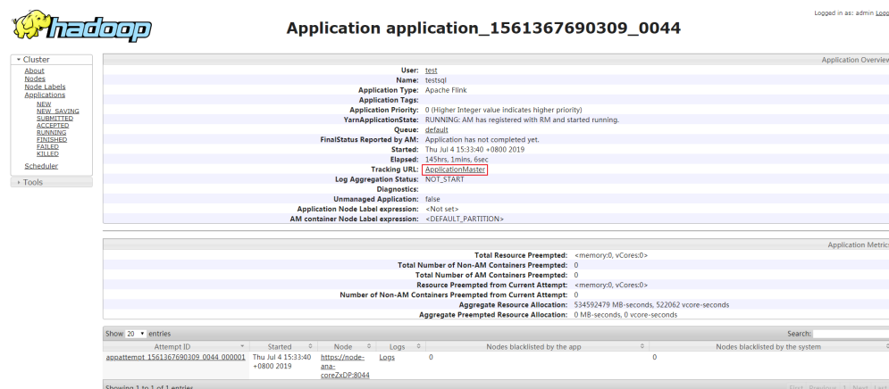
图 5-10 application
