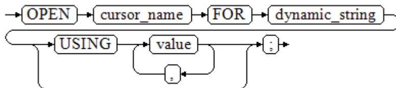
图 13-8 open_for::=
