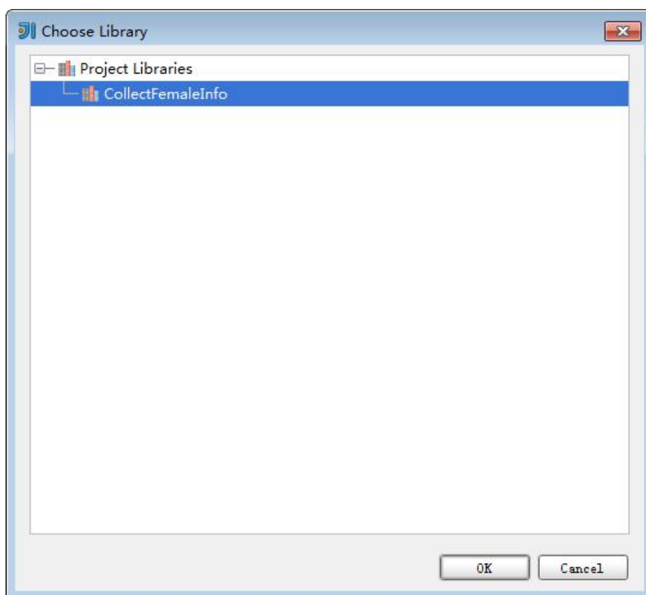
图 14-40 Choose Library
