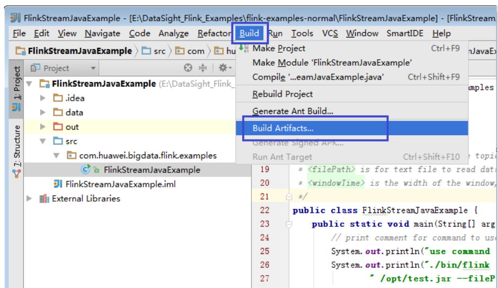
图 5-35 Build Artifacts
