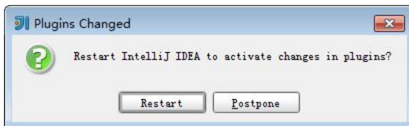
图 14-22 Plugins Changed
