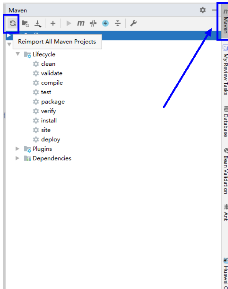
图 18-13 reimport projects
