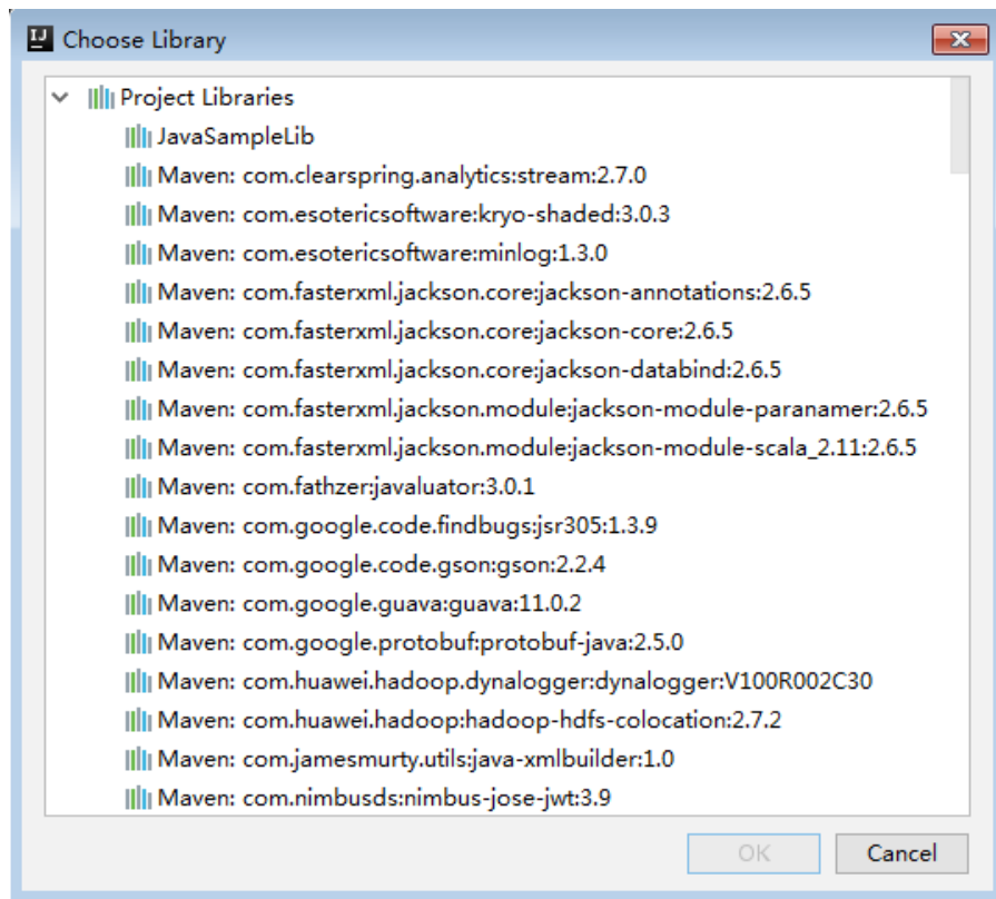
图 27-43 Choose Libraries
