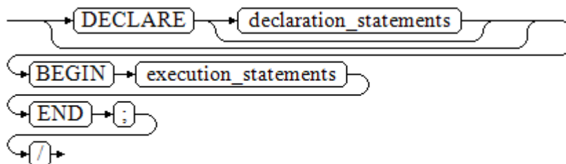
图 9-2 anonymous_block::=
