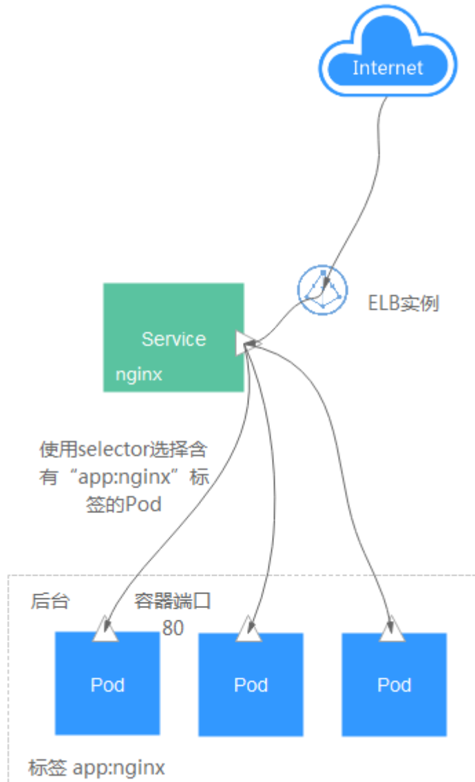
图 11-3 LoadBalancer Service
