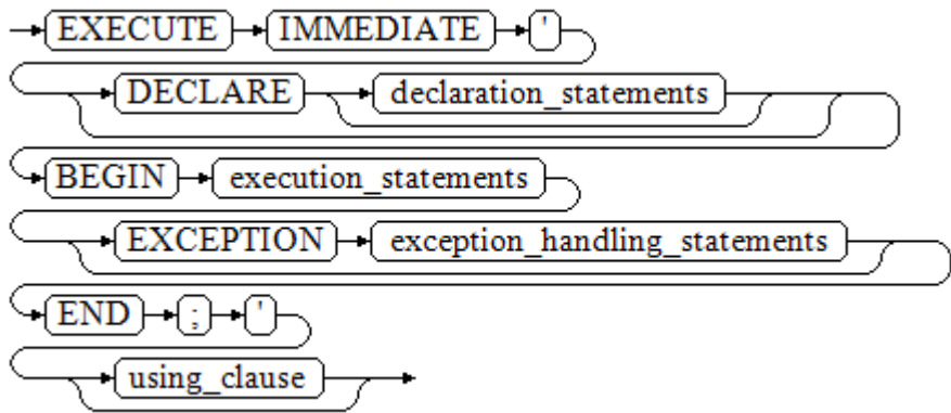
图 10-13 call_anonymous_block::=
