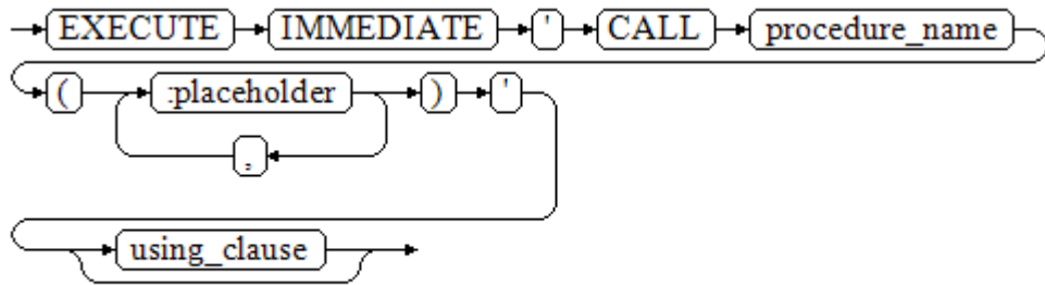
图 9-11 call_procedure::=
