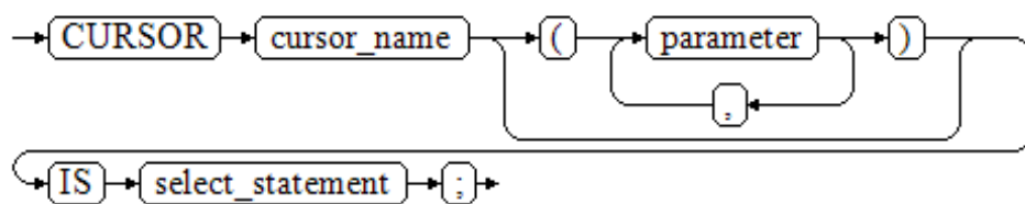
图 10-27 static_cursor_define::=
