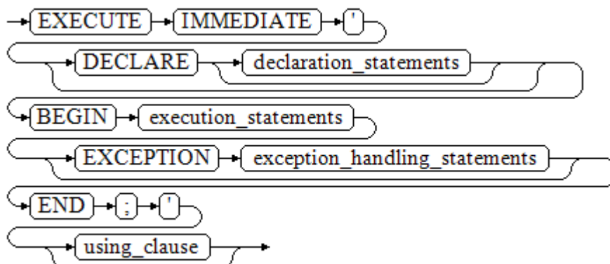
图 10-14 call_anonymous_block::=
