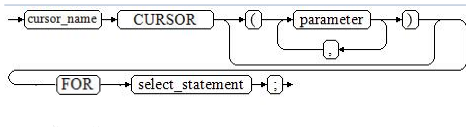
图 10-28 static_cursor_define::=
