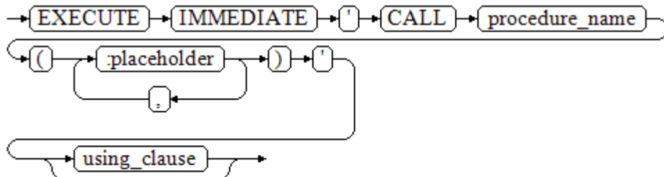
图 12-12 call_procedure::=
