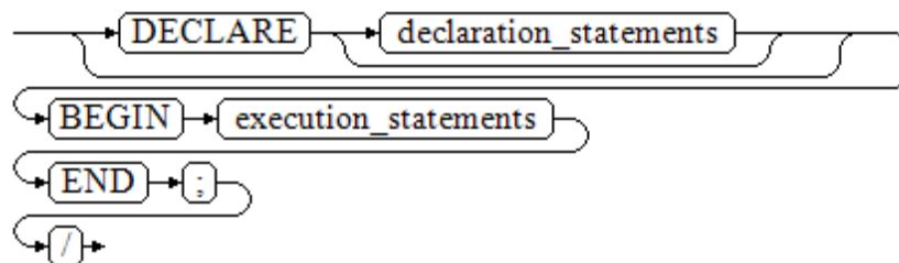
图 11-2 anonymous_block::=
