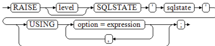
图 11-36 raise_sqlstate::=
