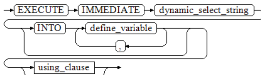
图 11-6 EXECUTE IMMEDIATE dynamic_select_clause::=
