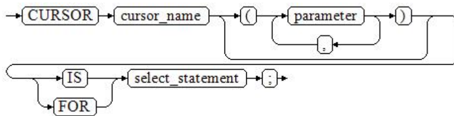
图 11-26 static_cursor_define::=
