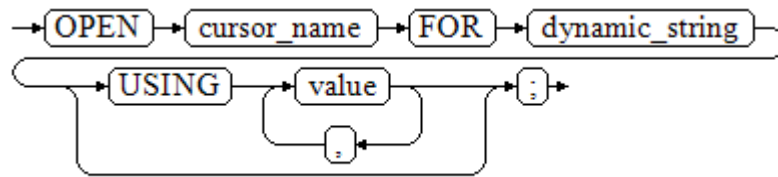
图 11-8 open_for::=
