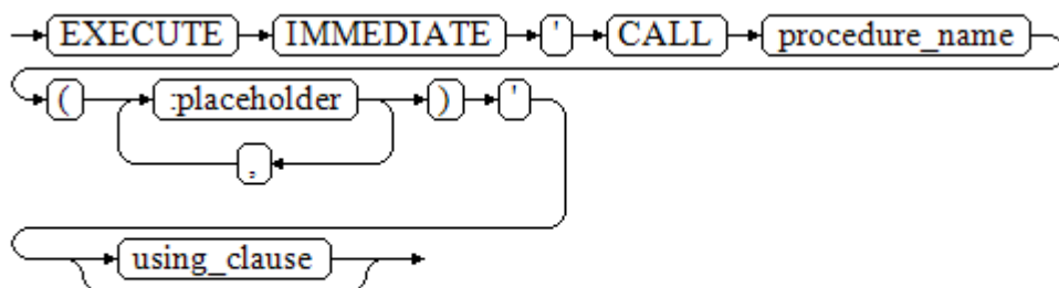
图 11-11 call_procedure::=
