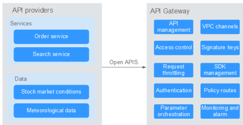
Figura 1-1 API opening
