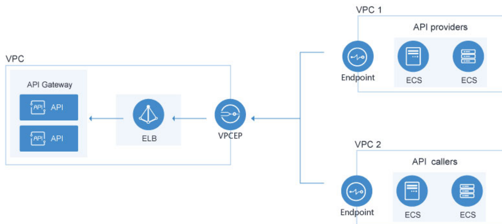
Figura 2-1 Cross-VPC access in the same region
