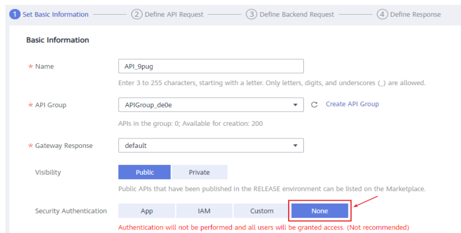
Figura 3-9 None authentication
