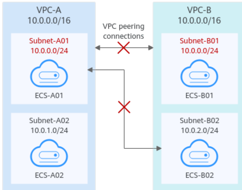
Figure 5-3 Networking diagram (IPv4)
