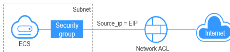
Figure 8-11 EIP network diagram
