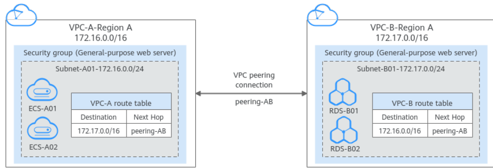
Figure 5-1 VPC peering connection network diagram
