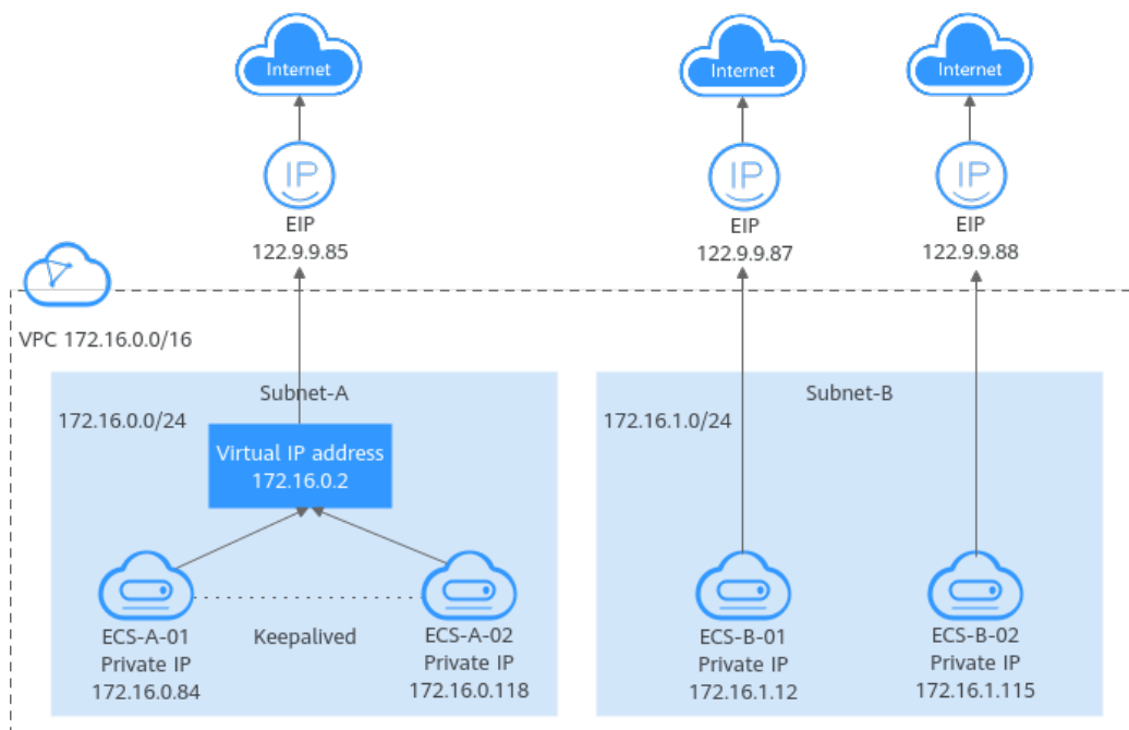
Figure 4-1 IP address architecture
