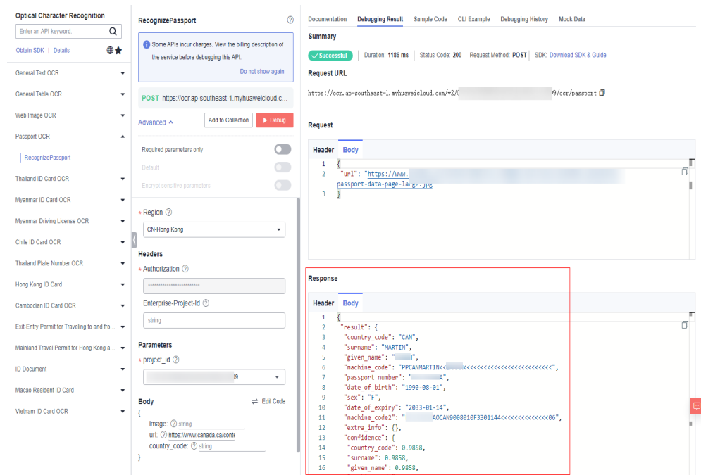
Figure 5-1 Recognition results
