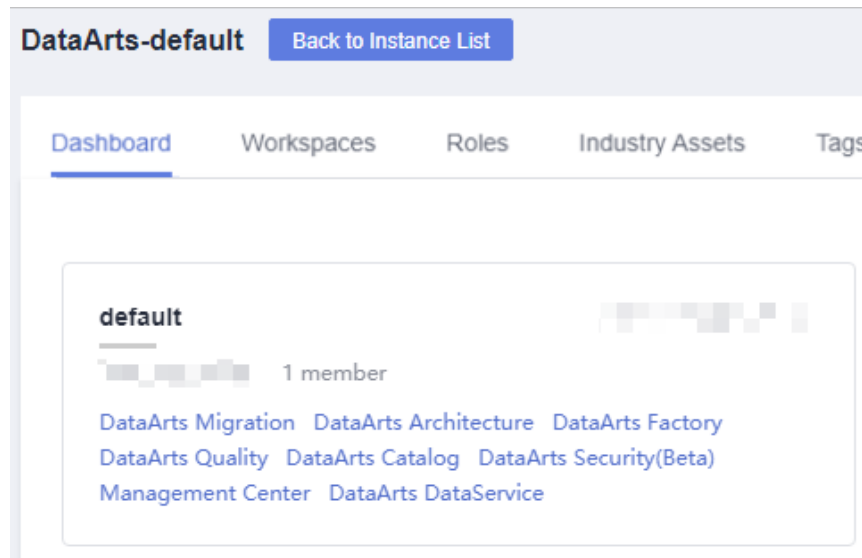
Figure 7-36 DataArts Quality
