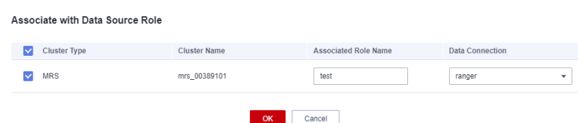
Figure 9-58 Associate
