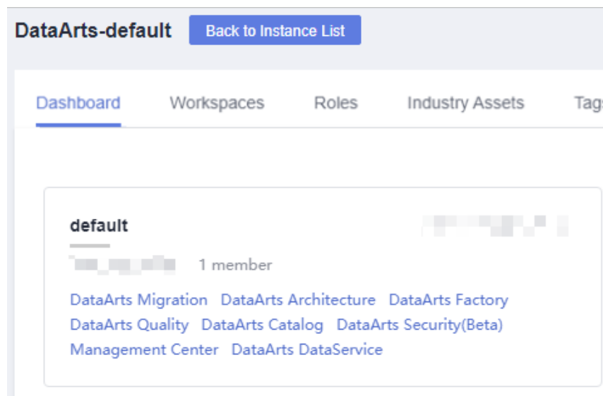
Figure 9-116 DataArts Security
