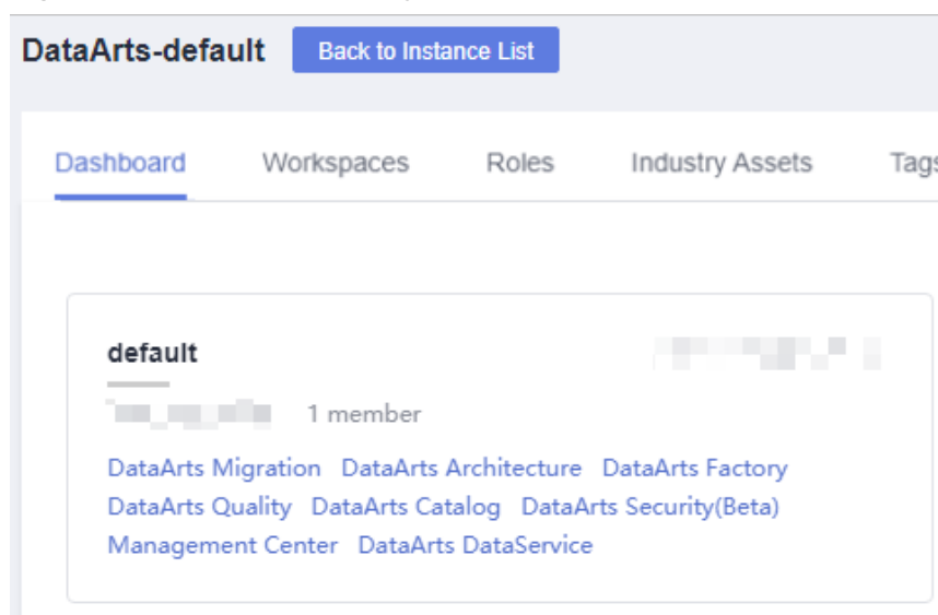
Figure 7-49 DataArts Quality
