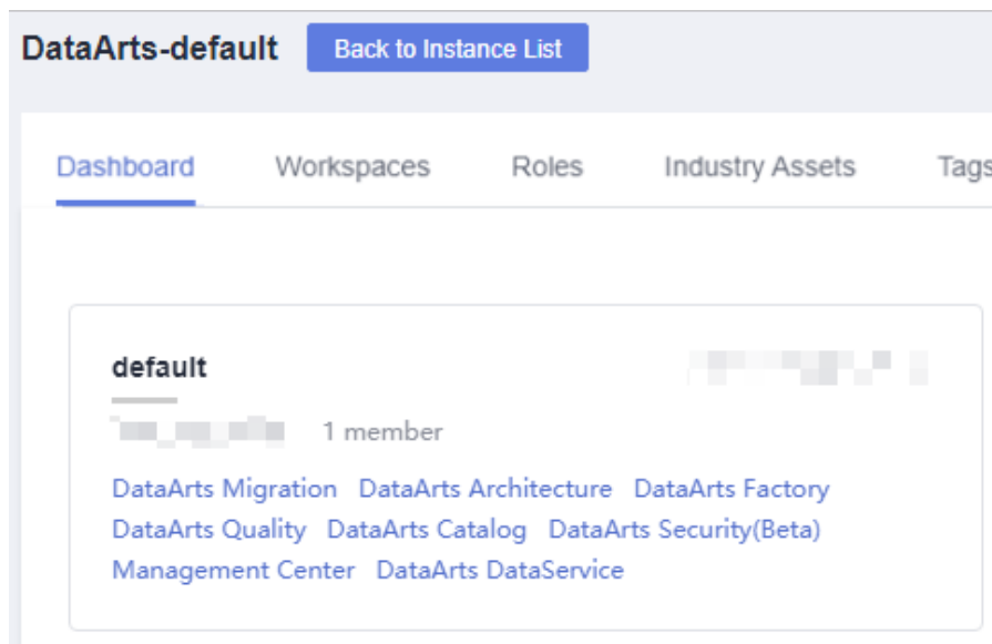
Figure 10-58 DataArts DataService
