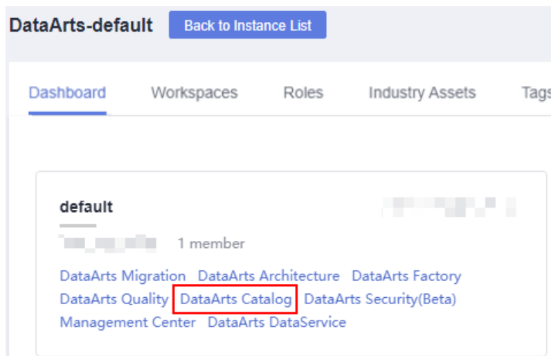
Figure 8-11 DataArts Catalog
