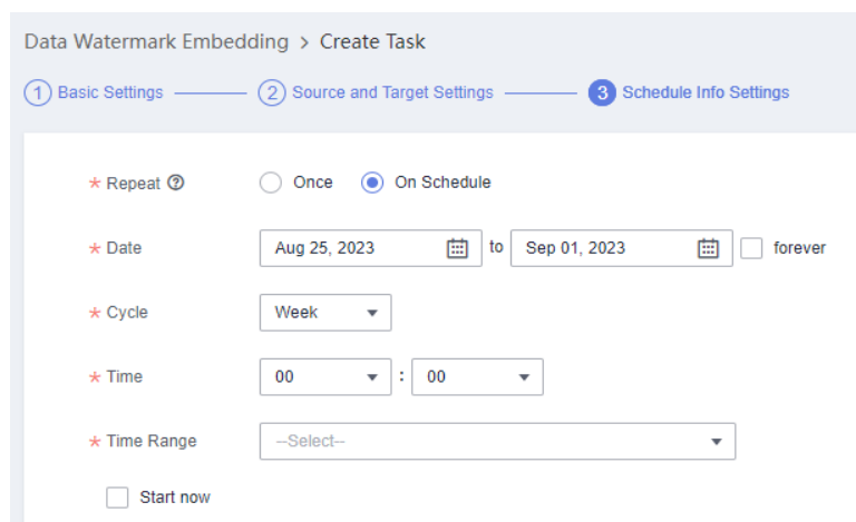
Figure 9-204 Configuring scheduling
