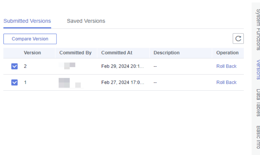
Figure 6-8 Comparing versions
