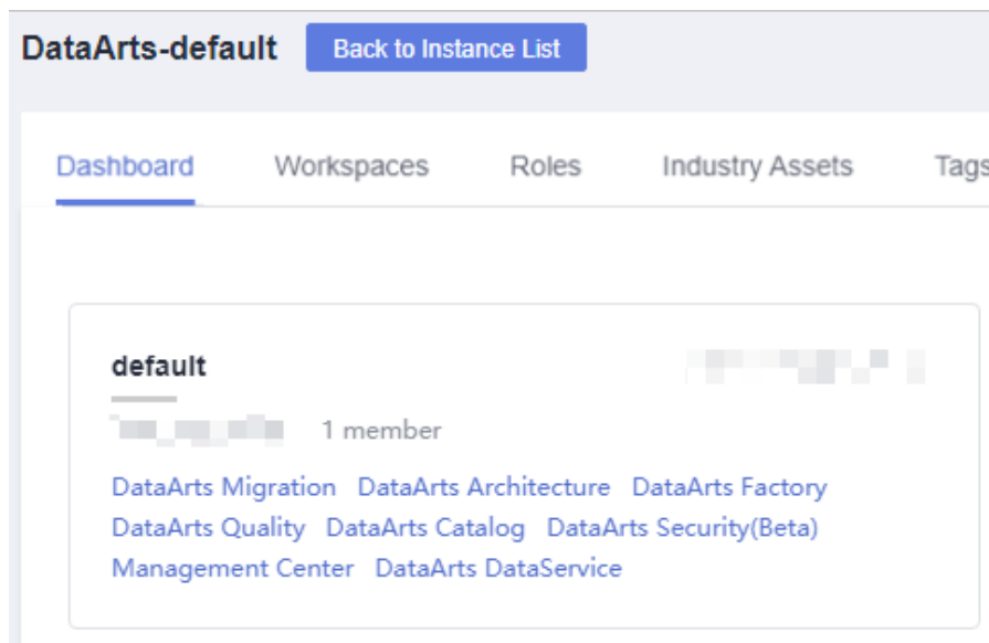
Figure 10-23 DataArts DataService
