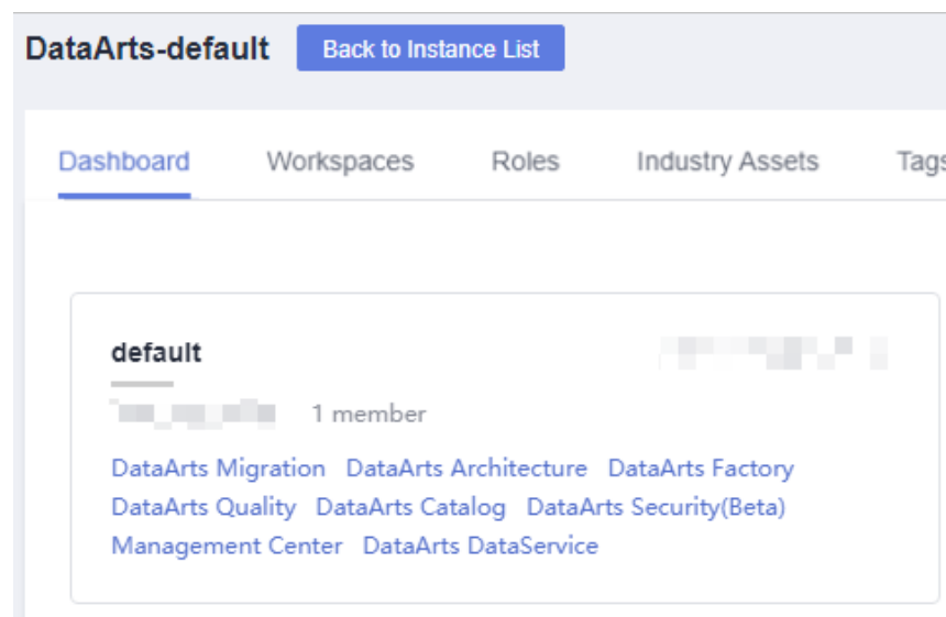
Figure 9-175 DataArts Security
