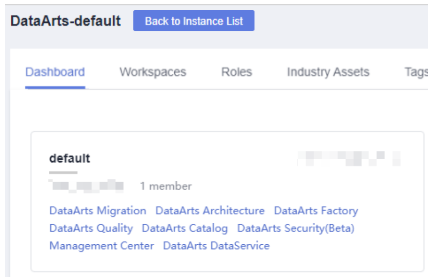
Figure 5-76 DataArts Architecture
