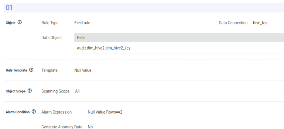
Figure 5-197 Quality rules
