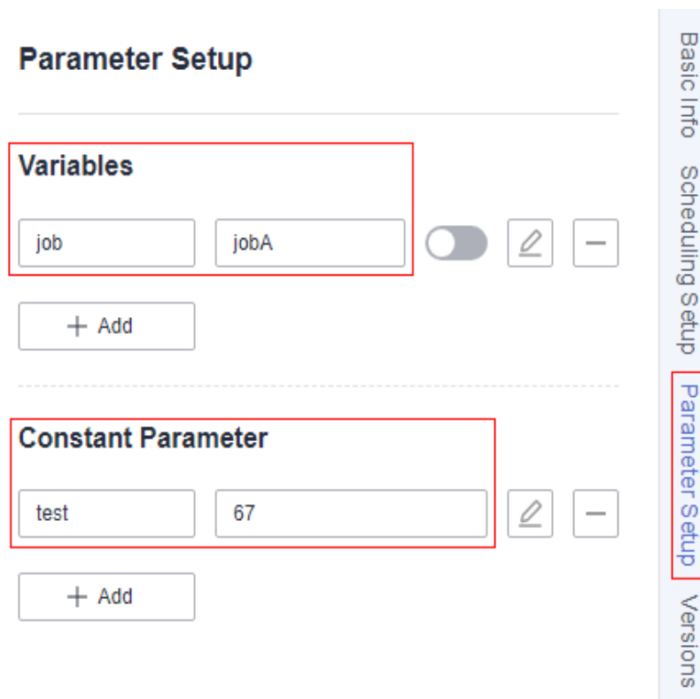
Figure 6-139 Job parameter.
