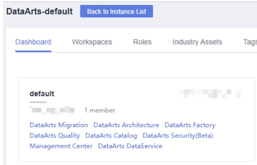
Figure 9-84 DataArts Security
