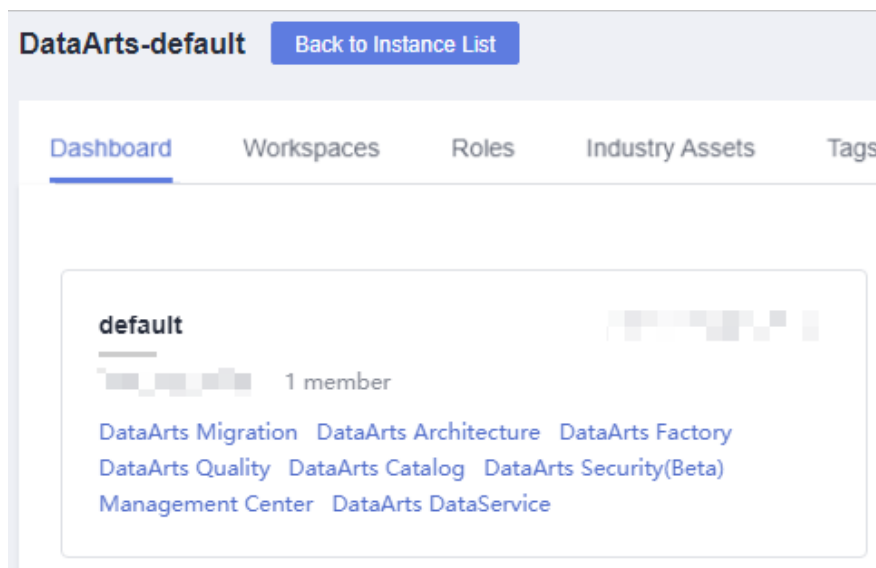
Figure 5-67 DataArts Architecture
