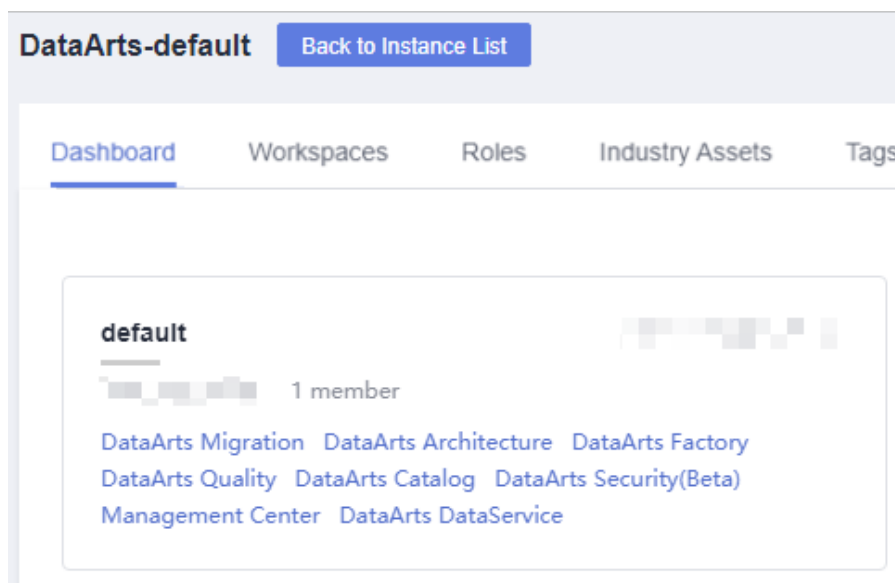
Figure 10-13 DataArts DataService
