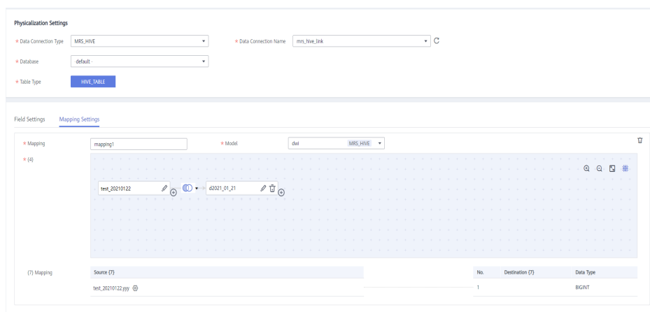
Figure 5-93 Mapping settings
