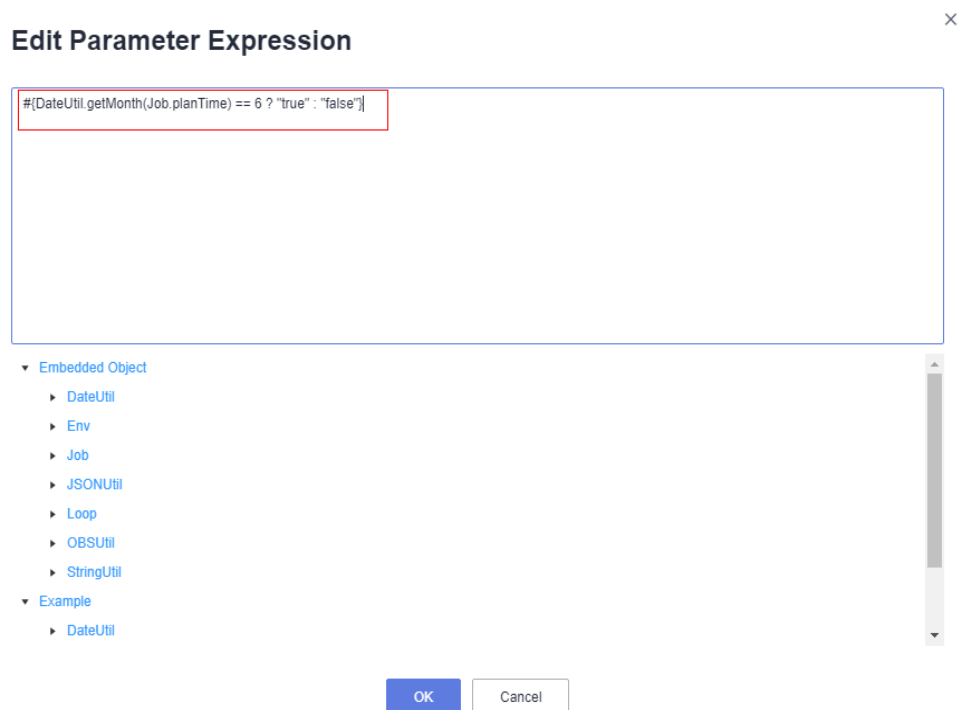
Figure 6-150 Condition expression
