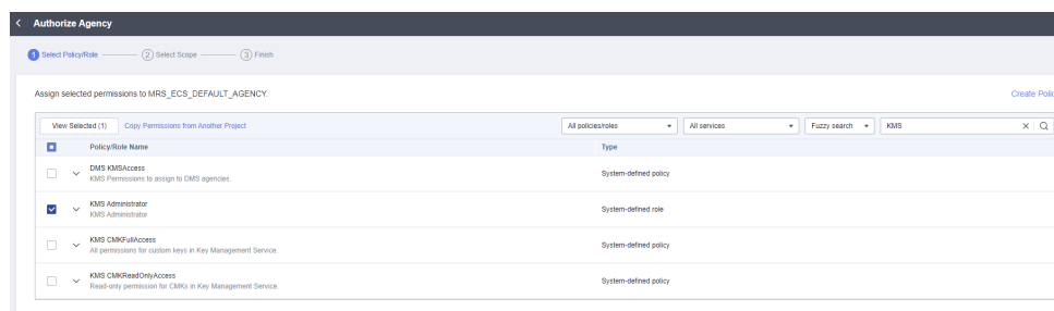
Figure 9-184 Selecting permissions
