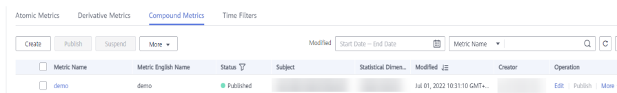
Figure 5-156 Compound metrics
