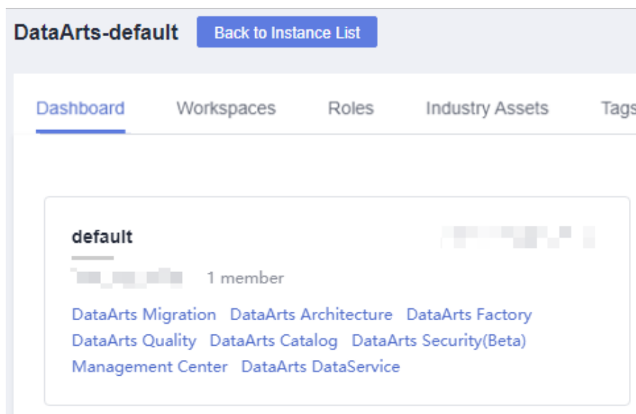
Figure 10-34 DataArts DataService
