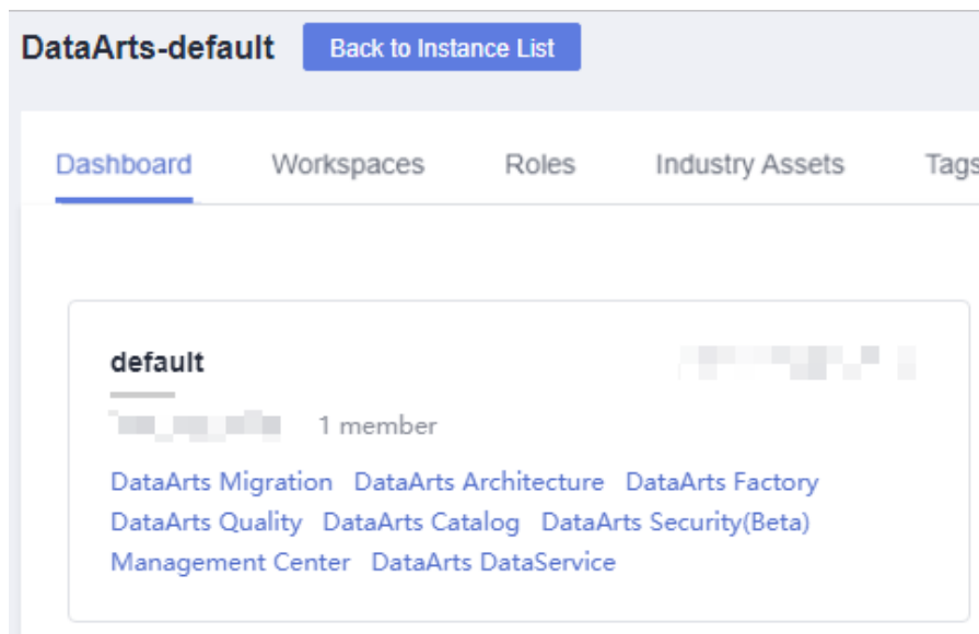
Figure 10-66 DataArts DataService
