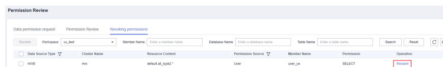
Figure 9-86 Revoking permissions
