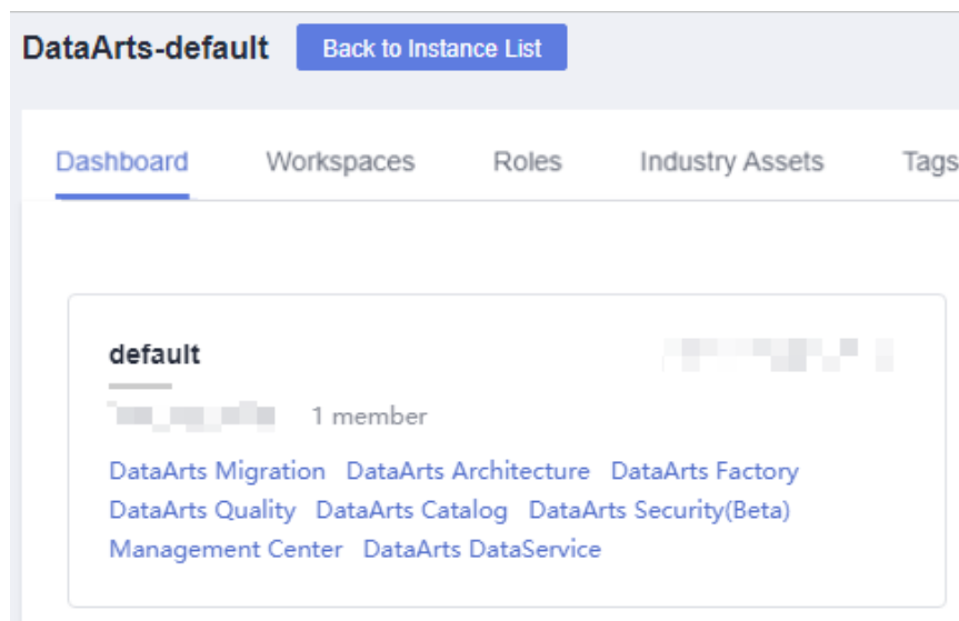
Figure 9-77 DataArts Security
