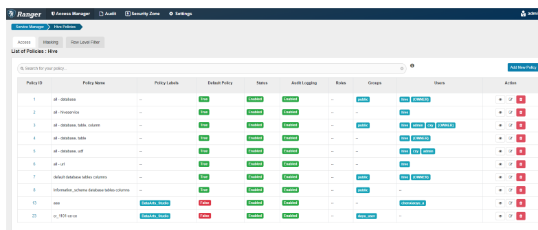
Figure 9-192 Policy list
