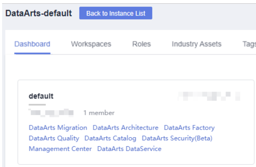
Figure 9-87 DataArts Security
