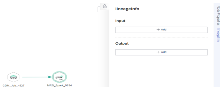
Figure 6-123 lineageInfo page
