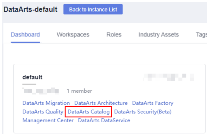
Figure 8-15 DataArts Catalog
