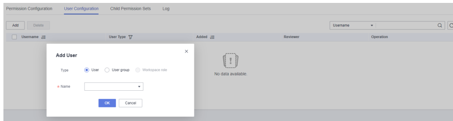
Figure 9-38 User Configuration
