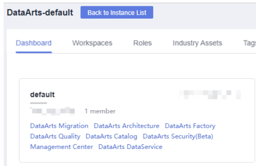
Figure 9-32 DataArts Security
