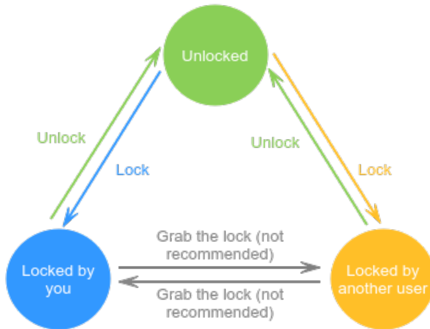
Figure 6-24 Lock statuses
