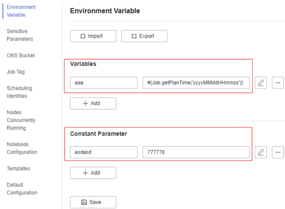
Figure 6-137 Environment Variable
