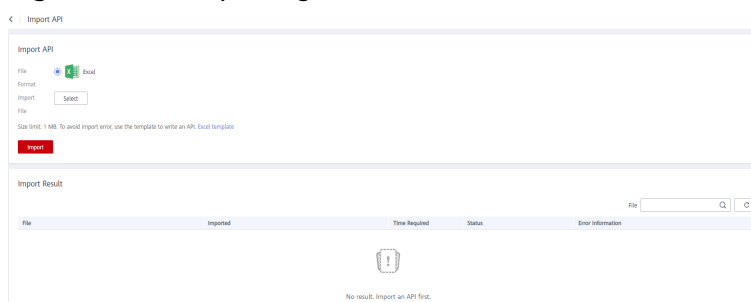
Figure 10-55 Importing APIs
