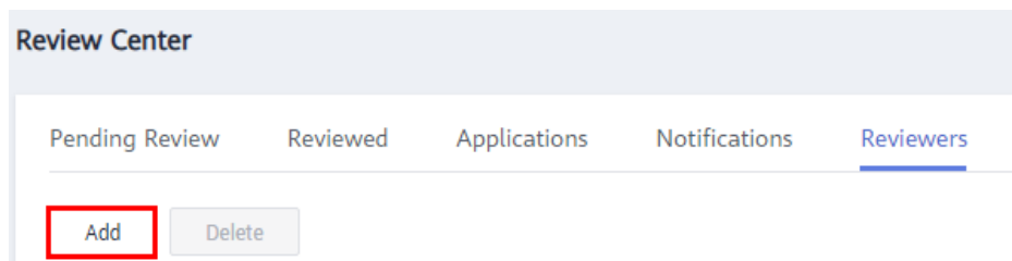
Figure 10-67 Adding reviewers
