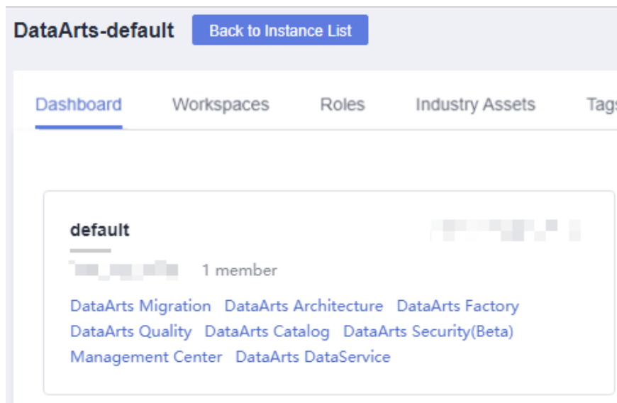
Figure 5-90 DataArts Architecture
