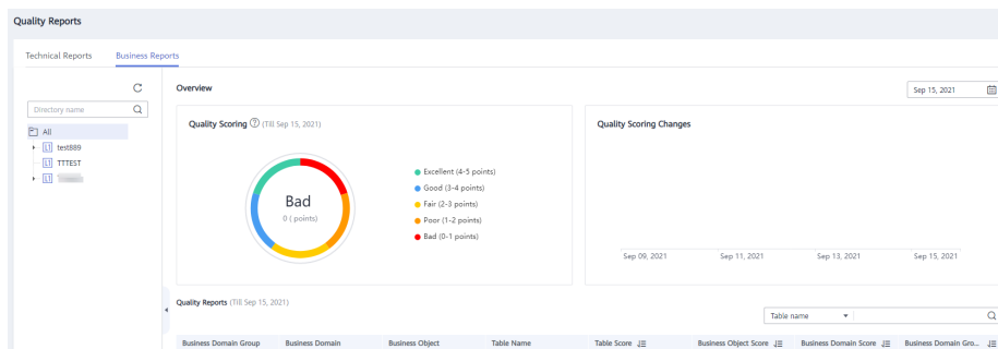
Figure 7-64 Business report
