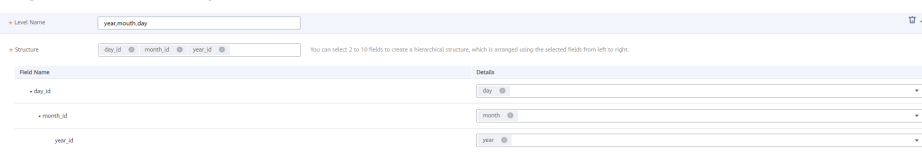
Figure 5-254 Layer 2
