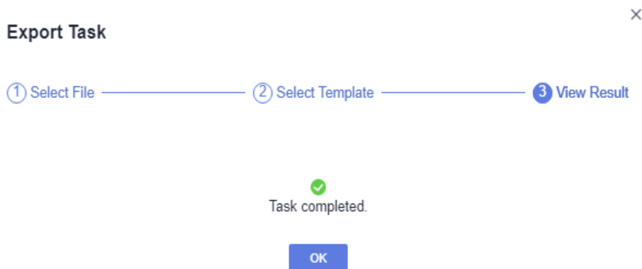
Figure 3-5 Export completed
