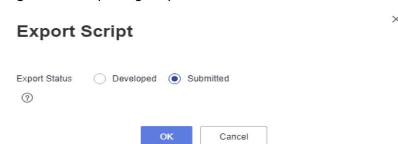
Figure 6-21 Exporting scripts
