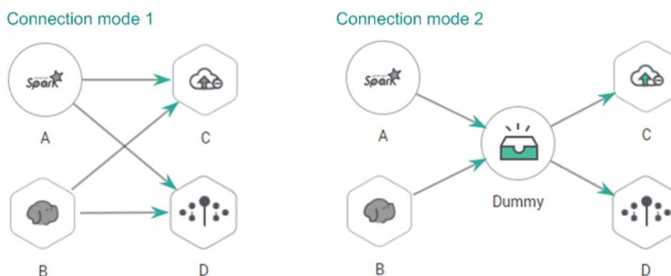
Figure 6-133 Connection modes
