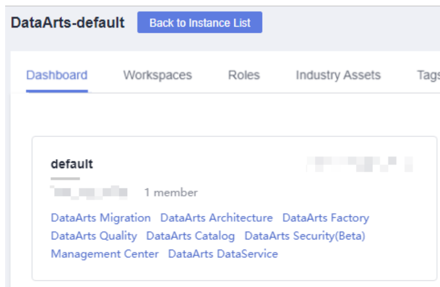
Figure 9-148 DataArts Security
