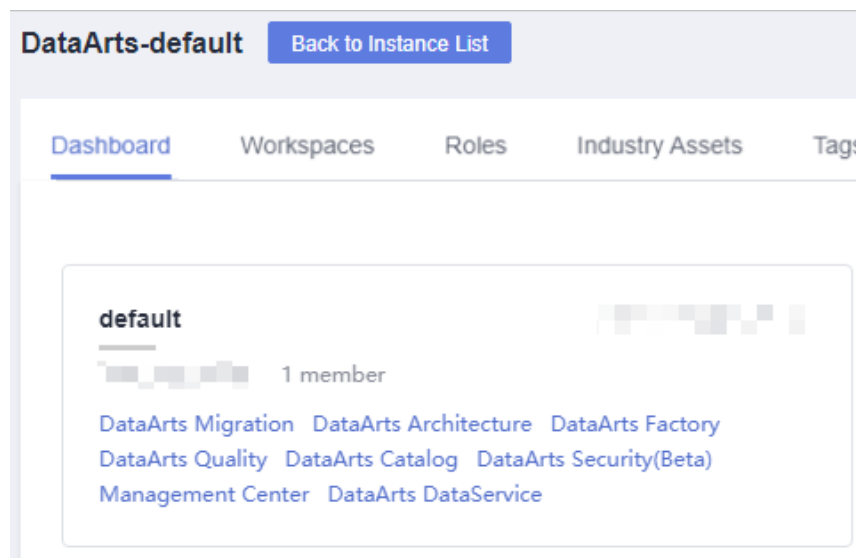
Figure 9-157 DataArts Security
