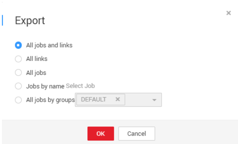
Figure 4-54 Export
