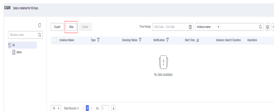
Figure 7-46 Stopping instances
