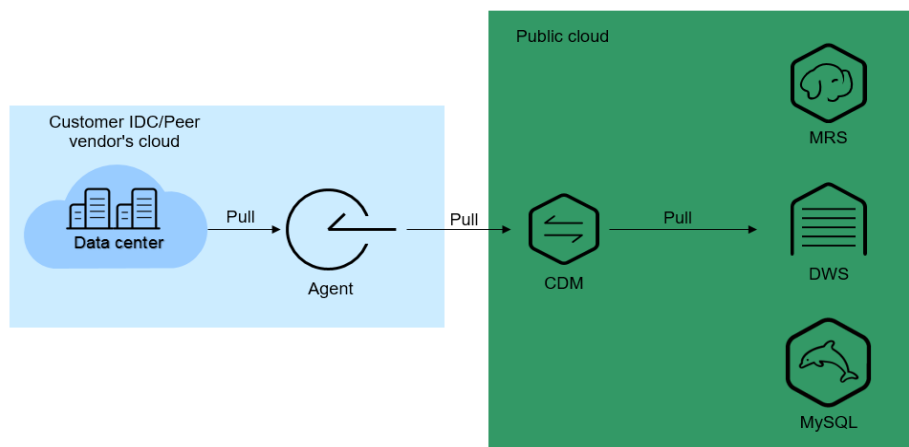
Figure 4-21 Scenario
