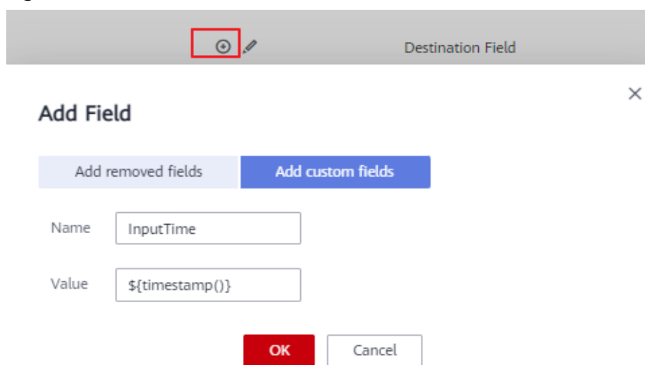
Figure 4-72 Add Field
