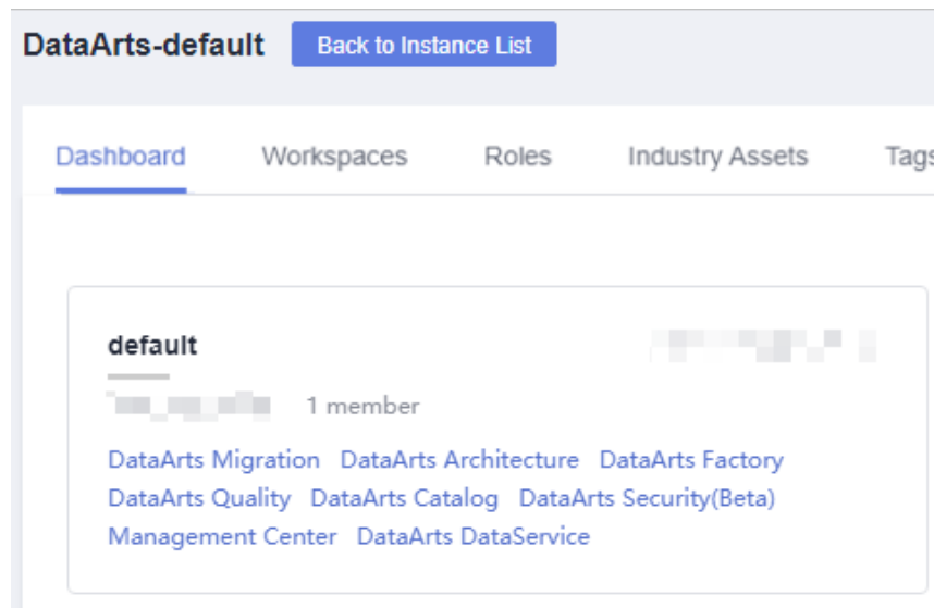
Figure 9-195 DataArts Security
