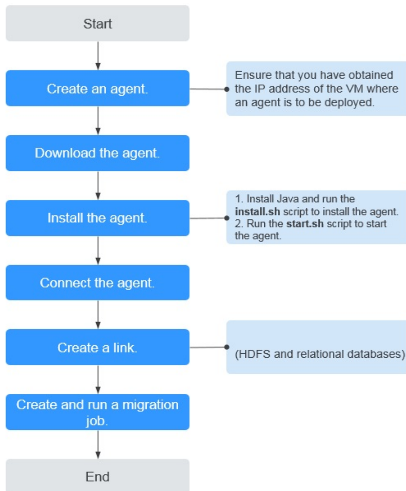
Figure 4-22 Process
