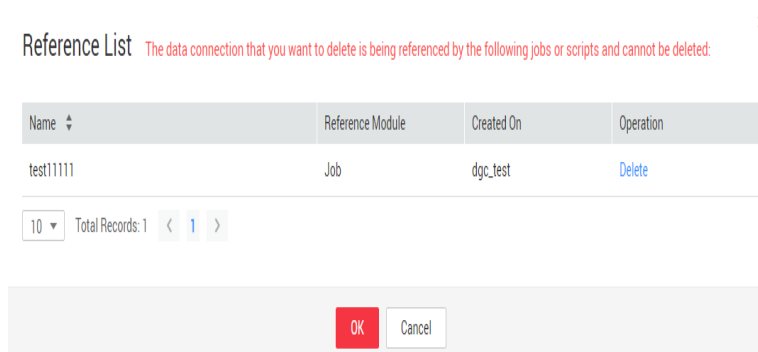
Figure 6-3 Reference List
