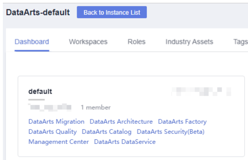
Figure 9-223 DataArts Security
