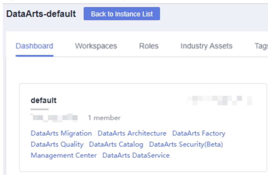
Figure 9-112 DataArts Security
