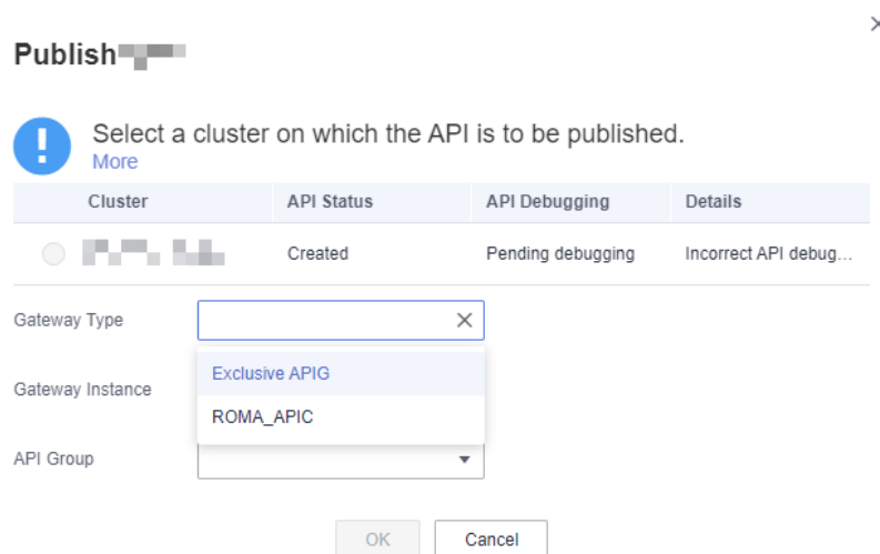
Figure 10-35 Publish
