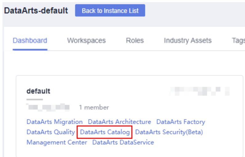
Figure 8-10 DataArts Catalog
