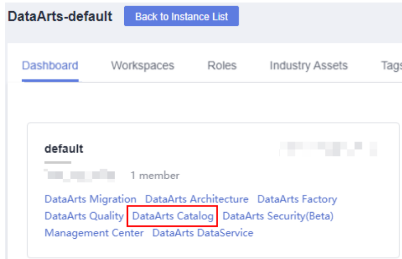
Figure 6-127 DataArts Catalog
