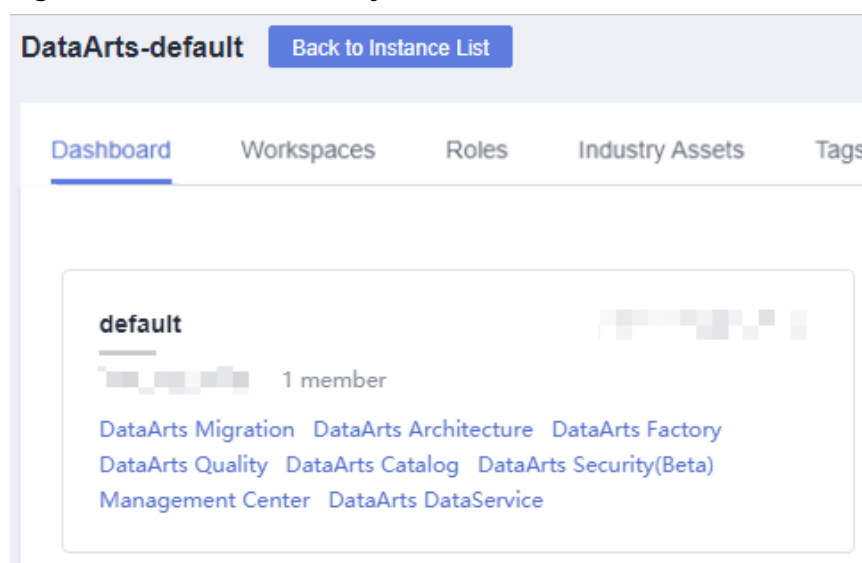
Figure 7-61 DataArts Quality
