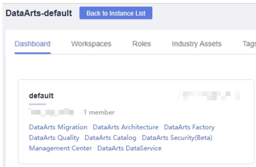
Figure 5-7 DataArts Architecture
