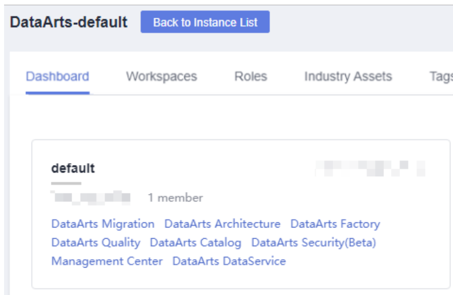
Figure 10-51 DataArts DataService
