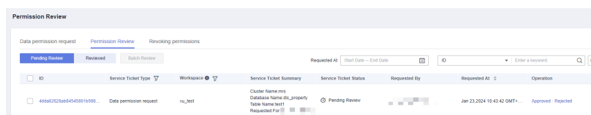
Figure 9-82 Permission Review
