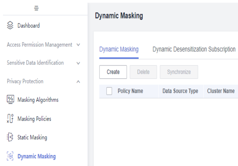
Figure 9-187 Dynamic Masking
