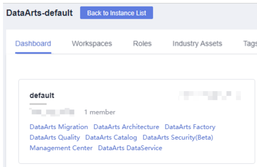
Figure 7-19 DataArts Quality
