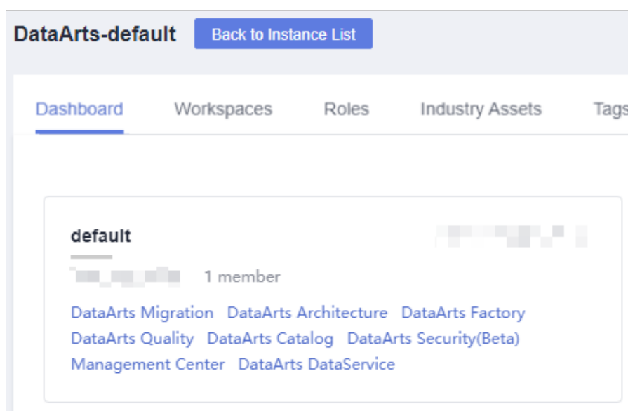
Figure 10-32 DataArts DataService
