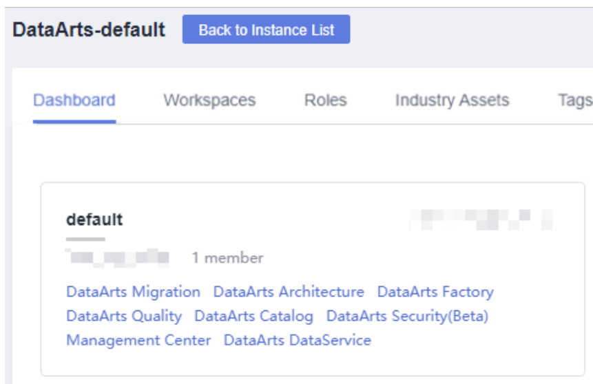
Figure 9-41 DataArts Security
