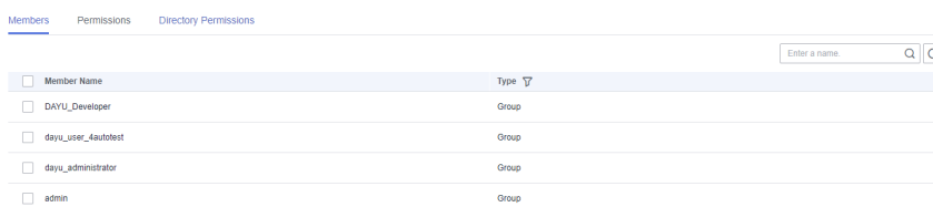
Figure 9-69 Members
