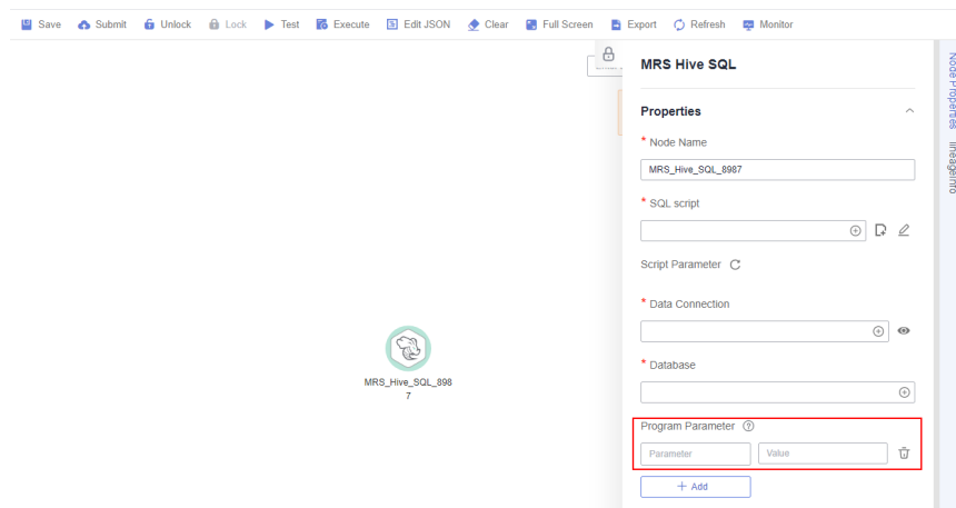
Figure 6-5 Program Parameter
