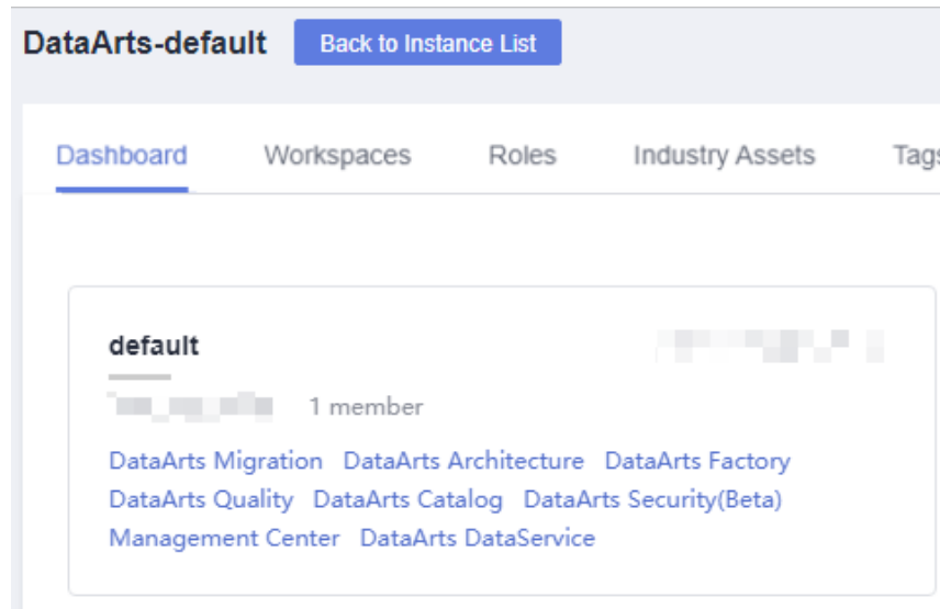
Figure 9-213 DataArts Security
