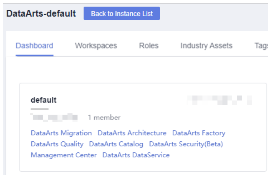
Figure 9-151 DataArts Security
