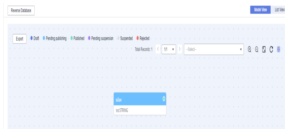
Figure 5-200 Model view
