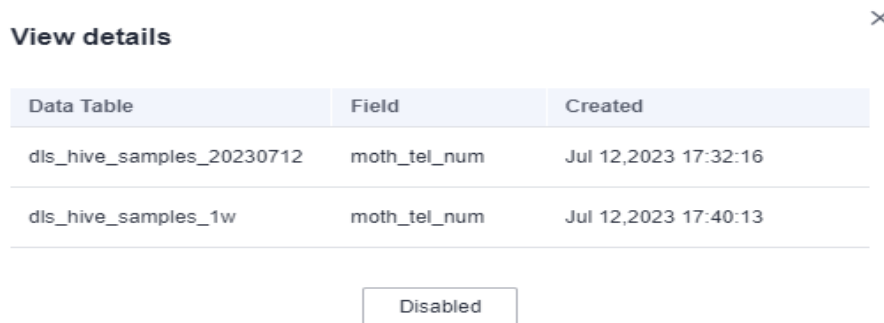
Figure 9-167 Viewing details
