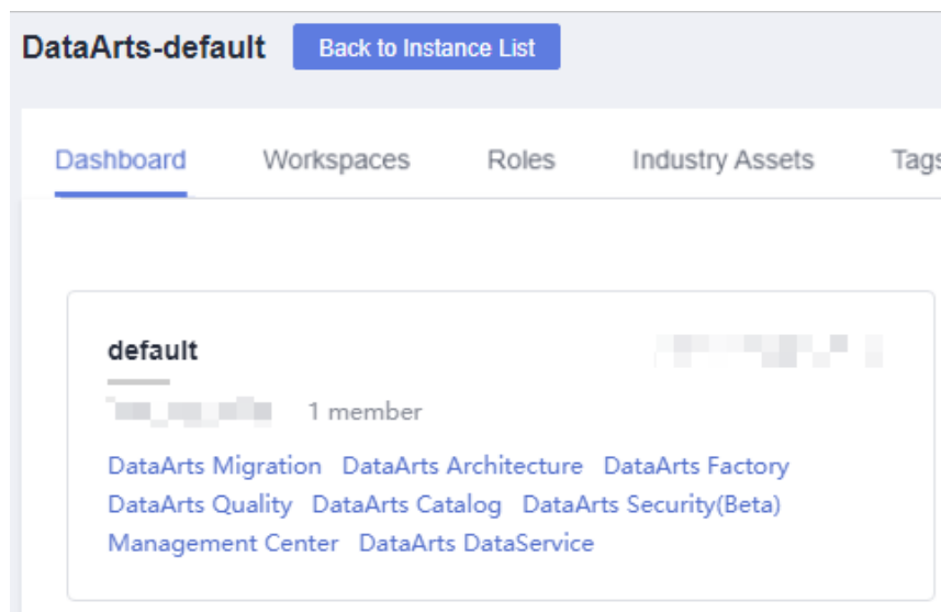
Figure 9-124 DataArts Security
