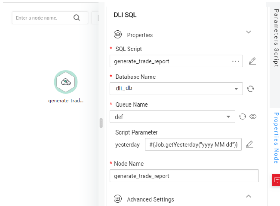
Figure 6-136 Node properties
