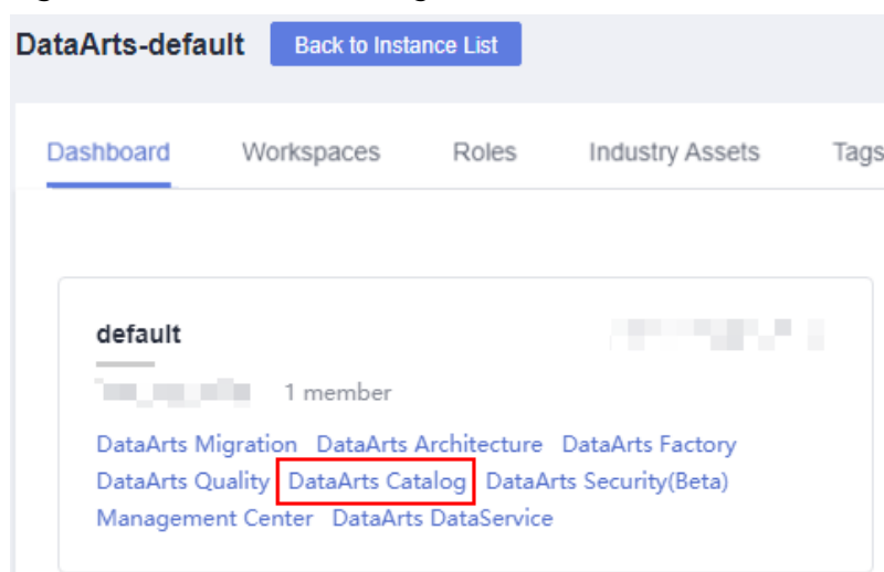
Figure 8-36 DataArts Catalog
