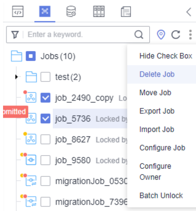
Figure 6-60 Deleting jobs
