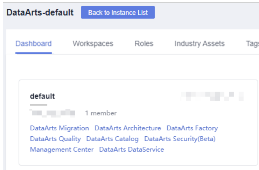
Figure 9-172 DataArts Security
