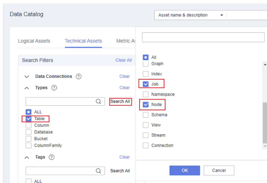
Figure 6-128 Selecting types
