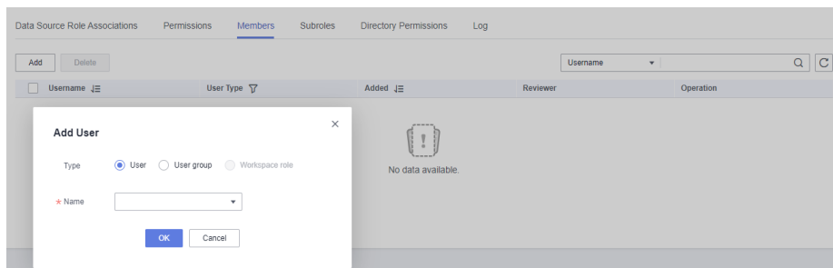
Figure 9-62 Members
