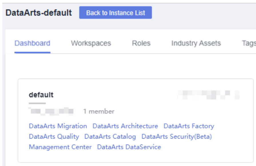
Figure 10-54 DataArts DataService
