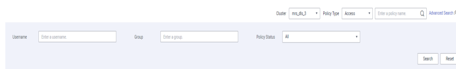
Figure 9-145 Advanced search
