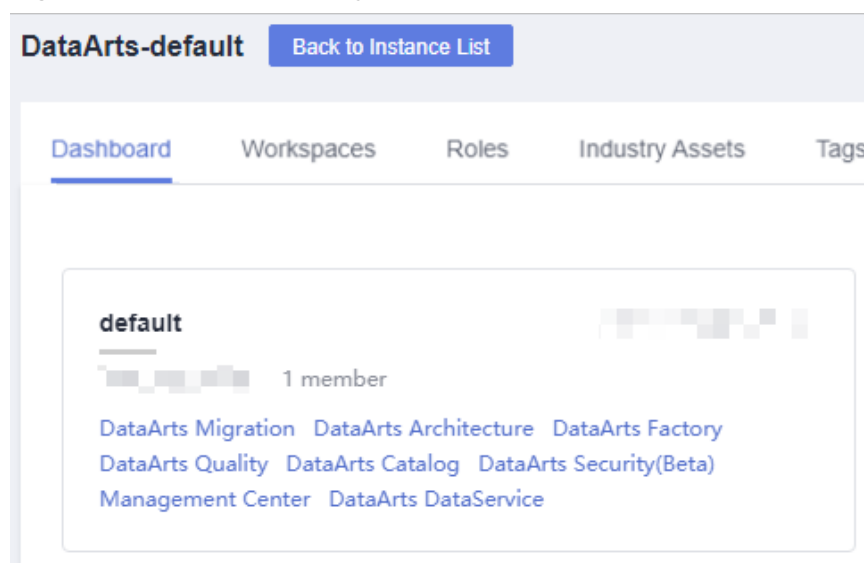
Figure 7-4 DataArts Quality
