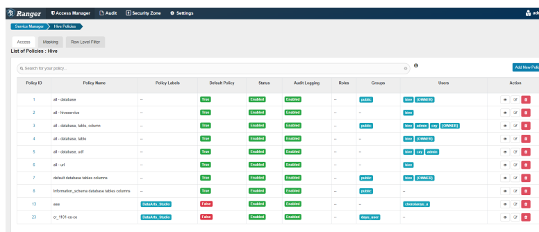
Figure 9-12 Policy list
