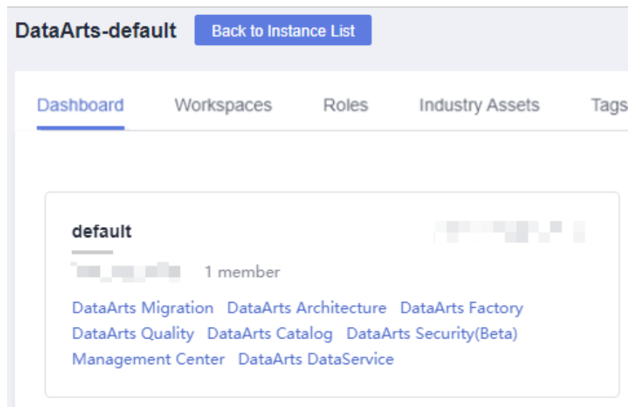
Figure 5-177 DataArts Architecture
