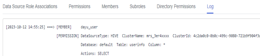
Figure 9-65 Viewing logs
