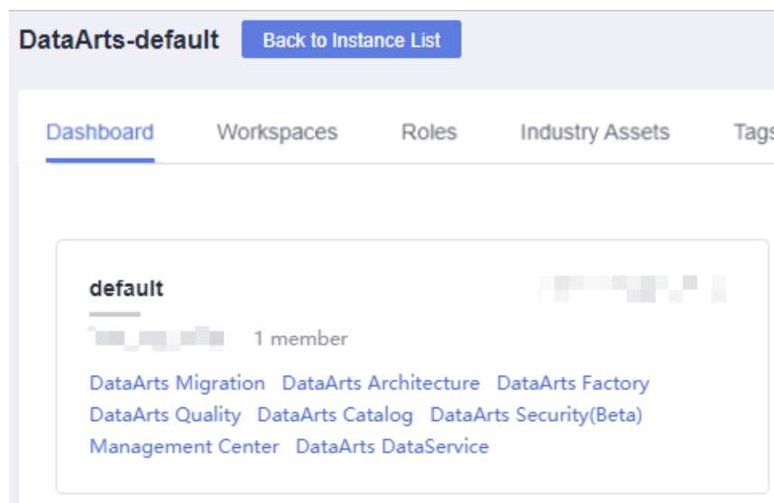
Figure 9-169 DataArts Security
