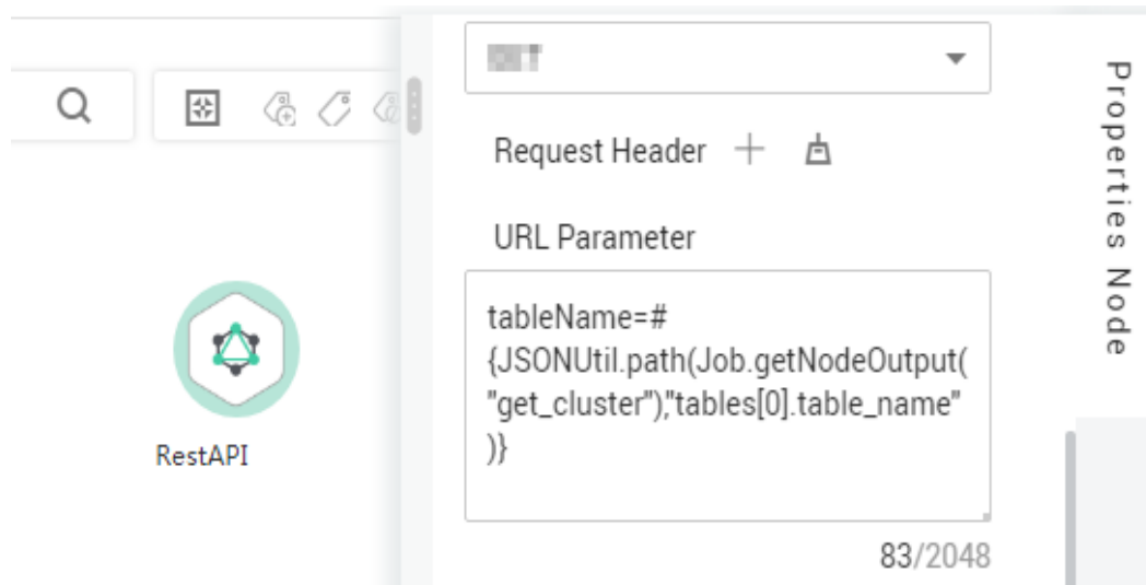
Figure 6-134 Expression example
