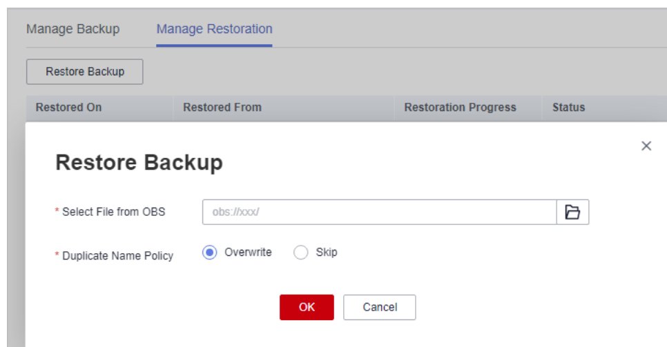
Figure 6-102 Restoring assets
