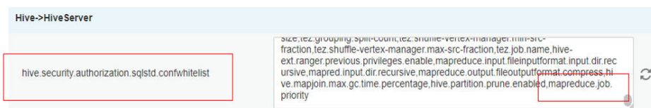
Figure 6-92 Configuring hive.security.authorization.sqlstd.confwhitelist
