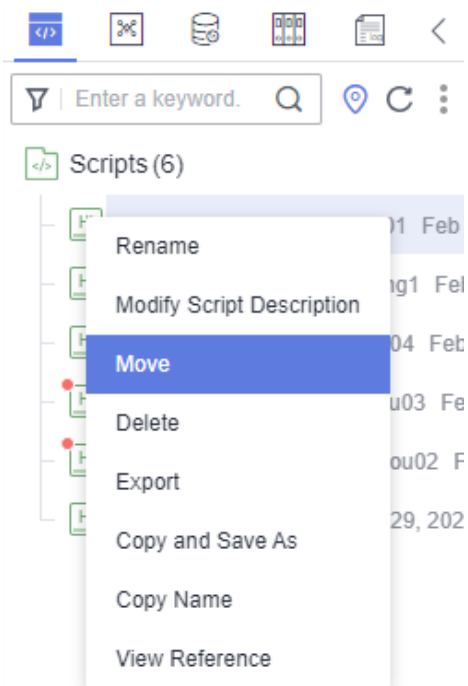
Figure 6-17 Selecting Move
