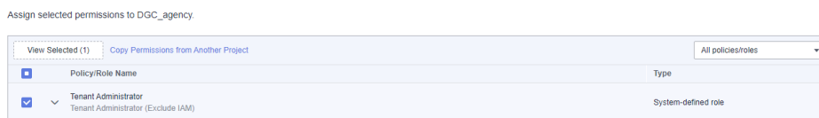
Figure 6-111 Assigning permissions
