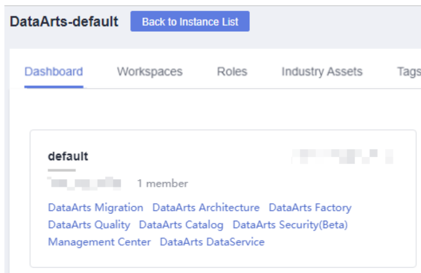
Figure 9-66 DataArts Security
