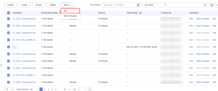
Figure 7-43 Running jobs
