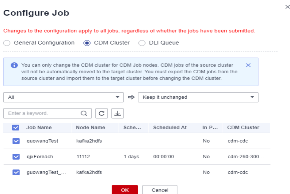
Figure 6-57 CDM Cluster
