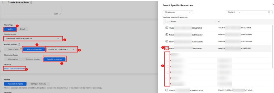
Figure 3-10 Configuring alarm rules for cluster nodes
