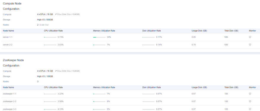
Figure 4-12 ClickHouse monitoring page
