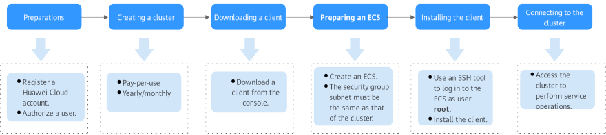
Figure 2-1 HBase usage process
