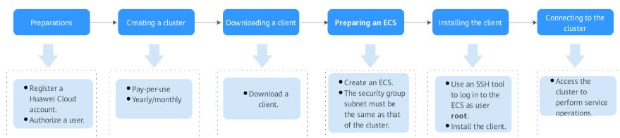
Figure 4-3 ClickHouse Usage Process
