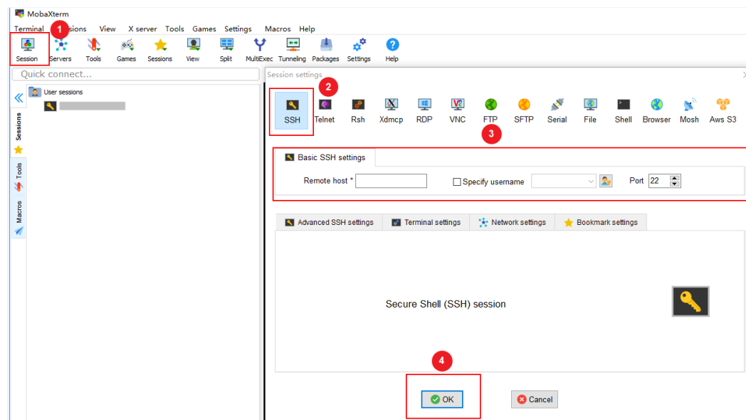
Figure 1-29 Logging to the VM
