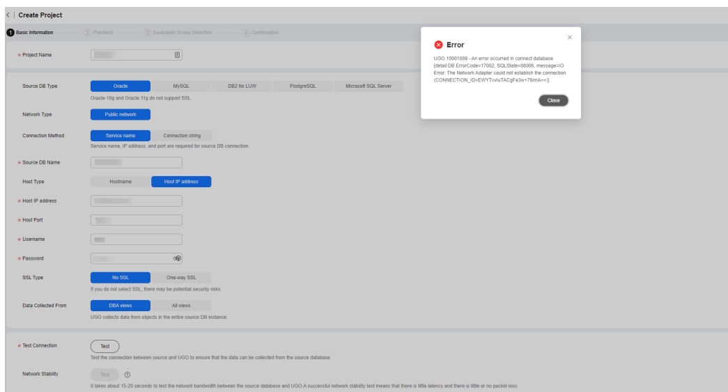
Figure 2-1 Error message
