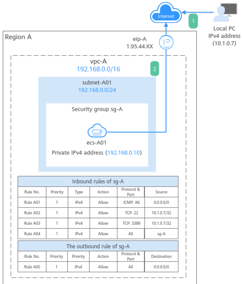
Figure 1-1 The architecture of an IPv4 network (VPC/ECS/EIP)
