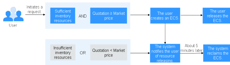
Figure 2-8 Lifecycle of a spot instance
