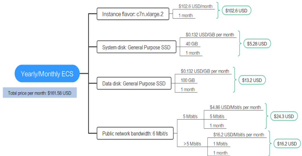
Figure 4-3 Total price for a yearly/monthly ECS
