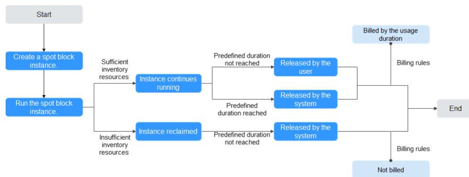
Figure 2-12 Lifecycle of a spot block instance
