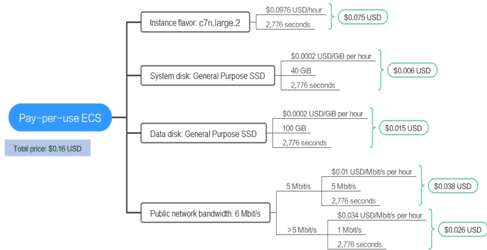
Figure 2-5 Total price for a pay-per-use ECS
