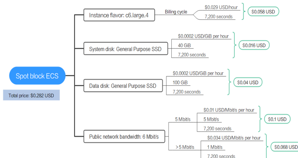
Figure 2-13 (Example 1) Total price for a spot block instance
