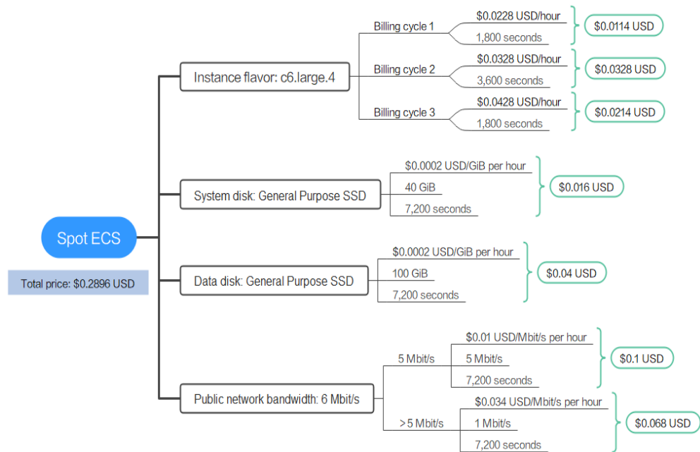
Figure 2-9 Total price for a spot instance
