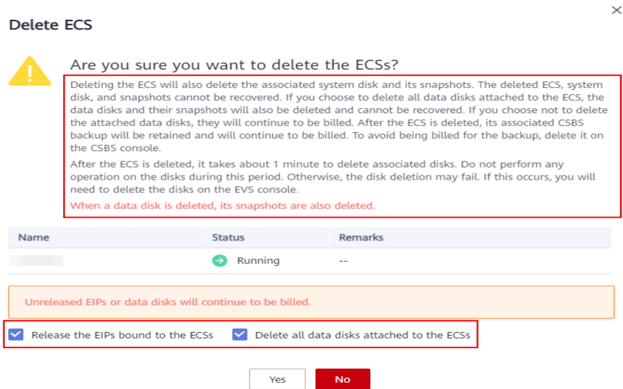
Figure 11-2 Deleting pay-per-use ECSs
