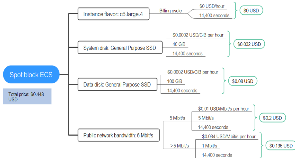
Figure 2-15 (Example 3) Total price for a spot block instance
