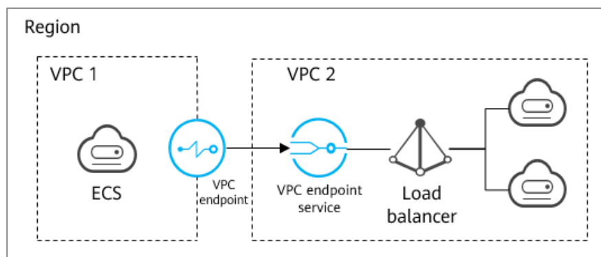
Figure 1-3 Cross-VPC connection
