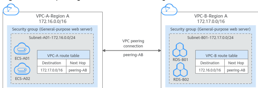
Figure 1-4 VPC peering connection network diagram
