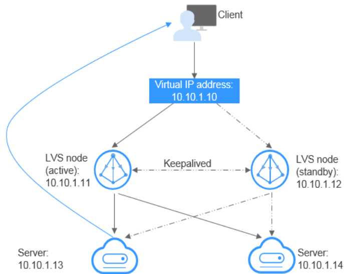
Figure 1-7 HA load balancing cluster
