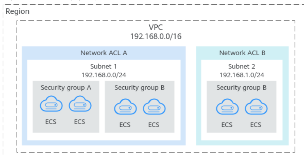
Figure 1-5 Security groups and network ACLs
