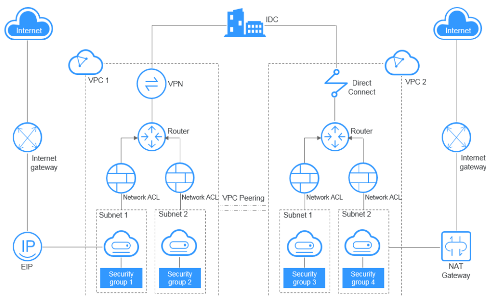
Figure 1-1 VPC components
