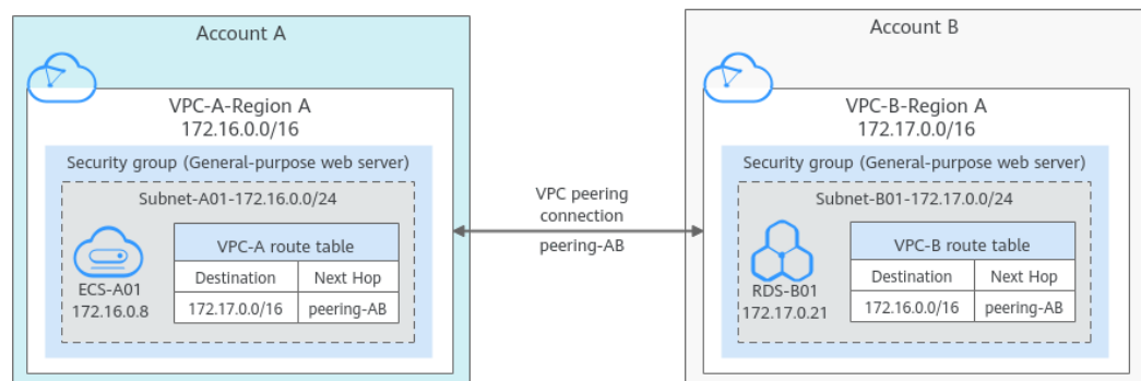
Figure 7-11 Networking diagram of a VPC peering connection between VPCs in different accounts
