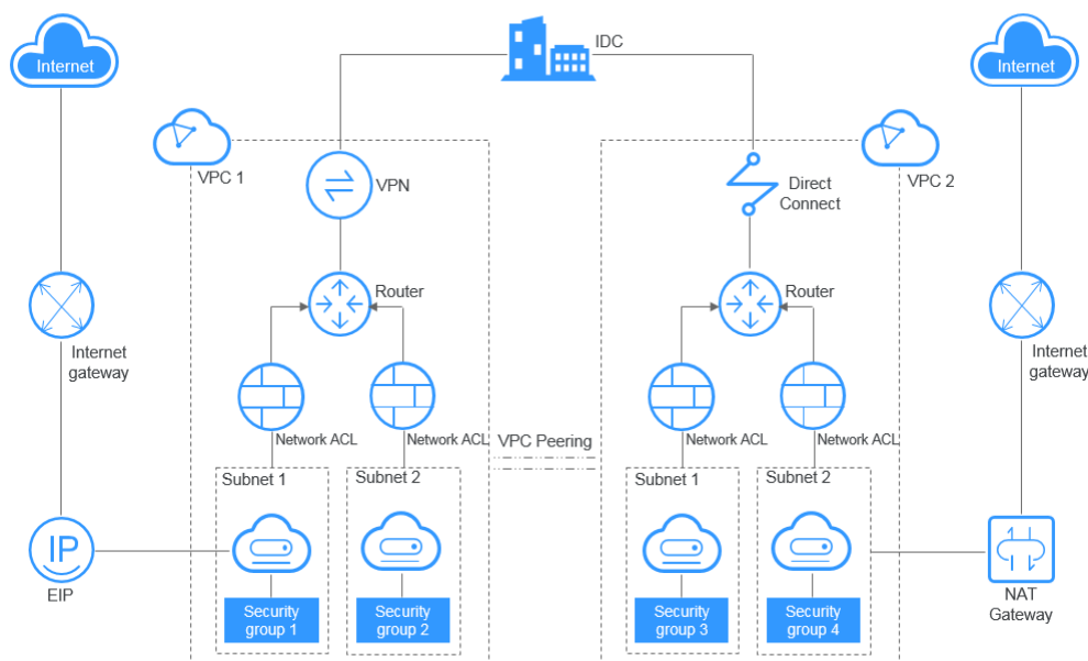
Figure 13-1 Product Architecture
