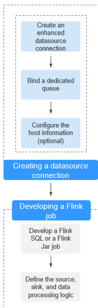
Figure 9-3 Datasource connection analysis process
