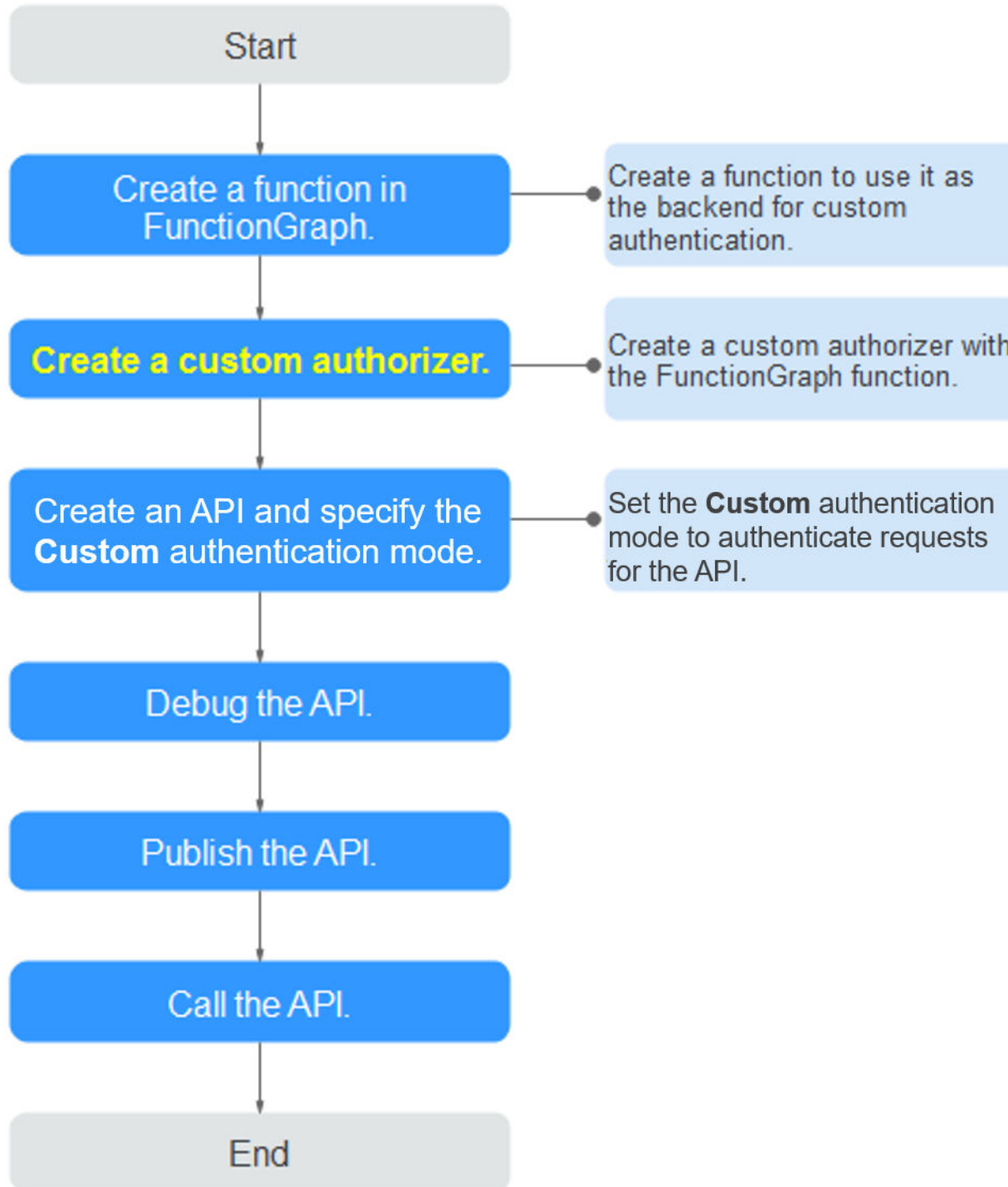
Figure 4-6 Calling APIs through custom authentication
