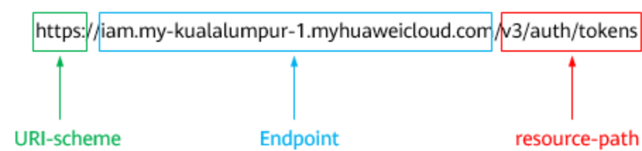
Figure 2-1 Example URI
