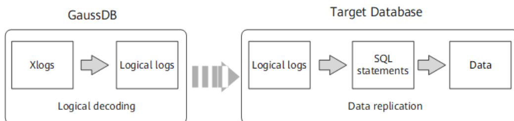
Figure 6-1 Logical replication
