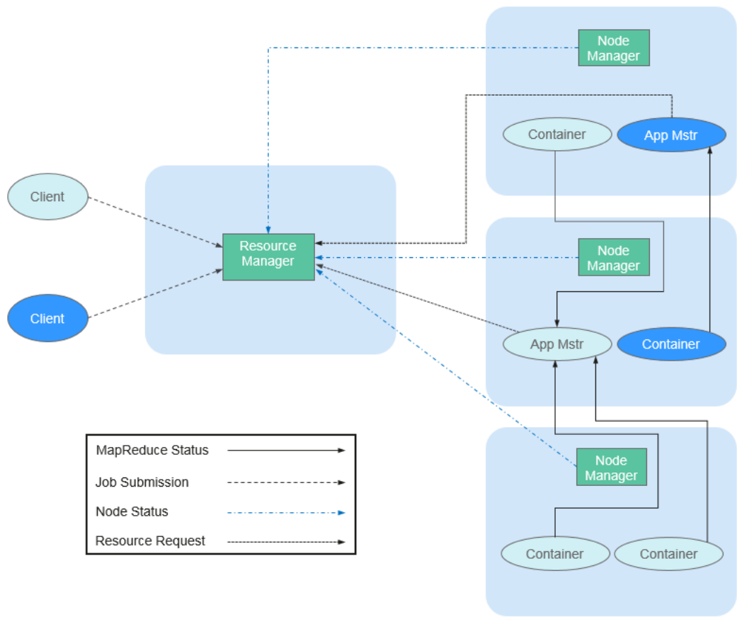
Figure 1-127 Architecture
