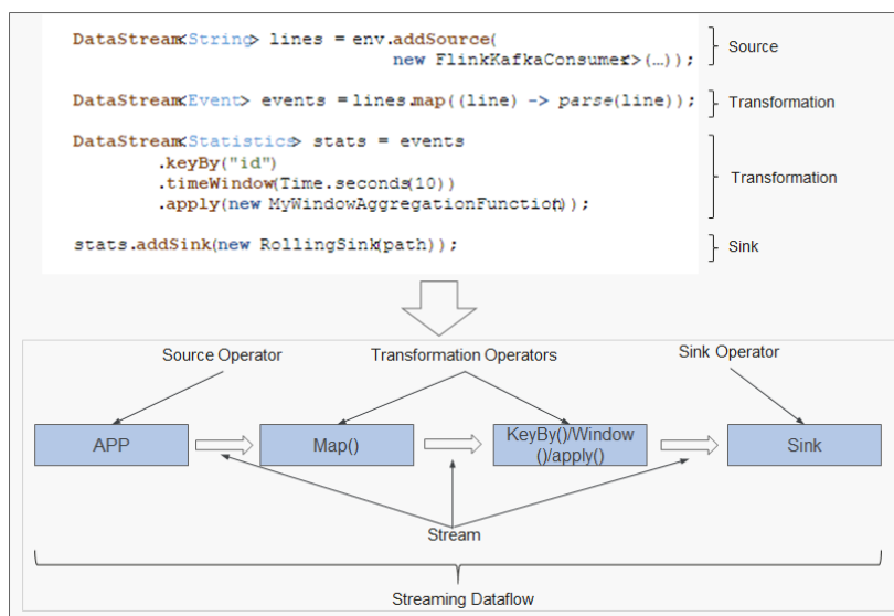
Figure 1-12 Example of Flink DataStream
