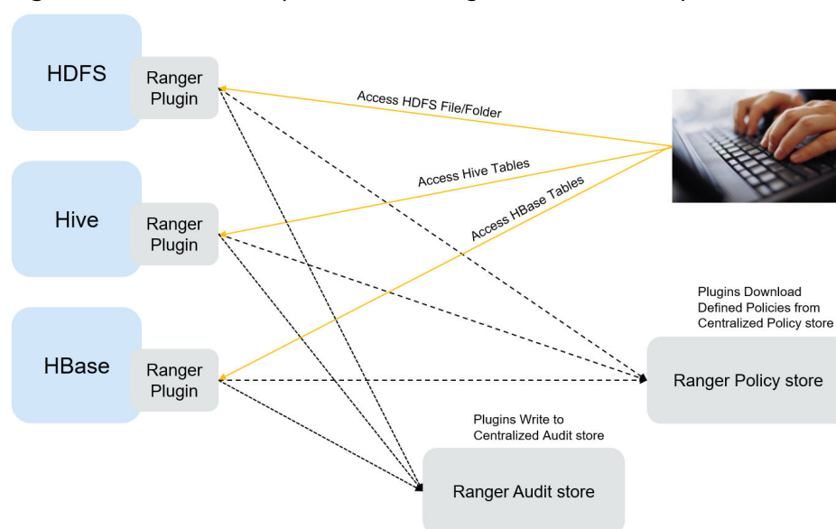
Figure 1-83 Relationships between Ranger and other components
