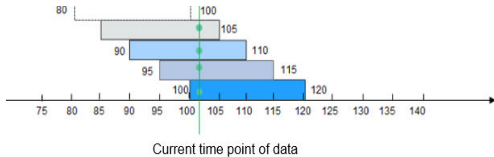
Figure 1-17 Original structure of a window
