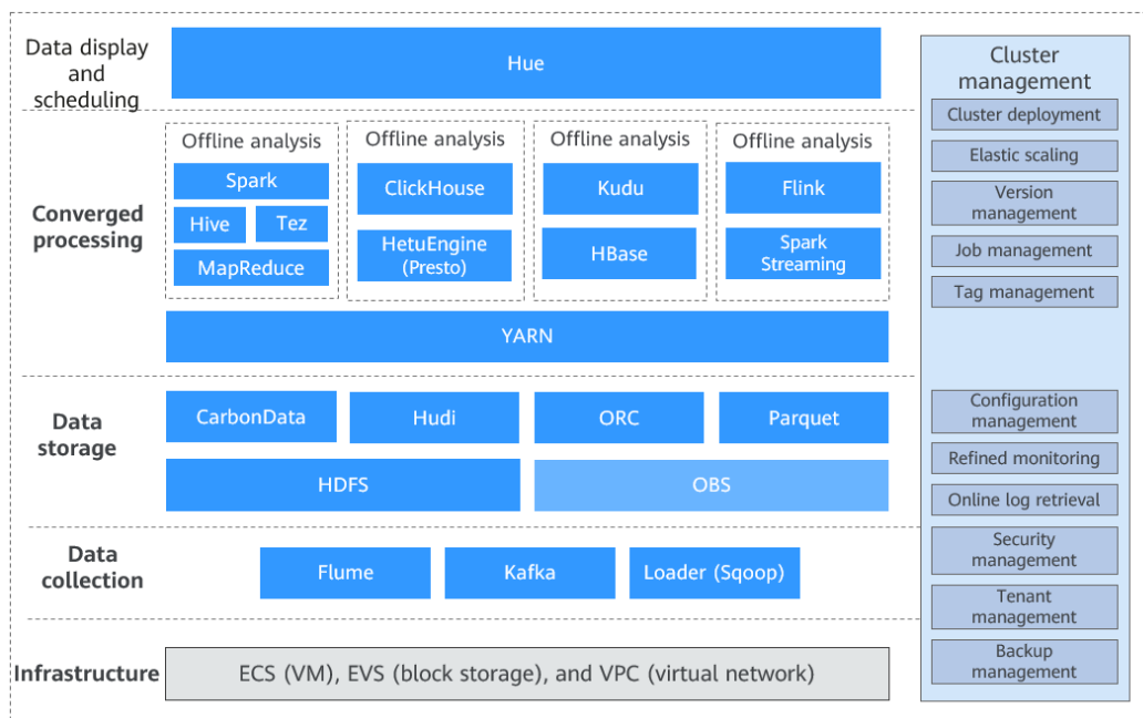
Figure 1-1 MRS architecture
