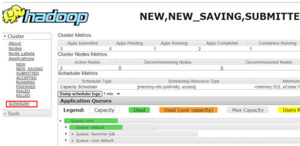
Figure 15-8 Queue resource usage on the Yarn page
