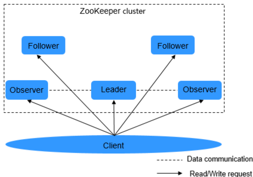
Figure 1-138 ZooKeeper architecture
