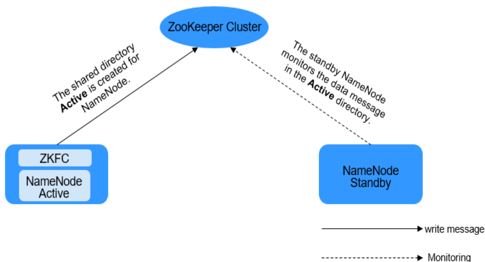
Figure 1-139 Relationship between ZooKeeper and HDFS
