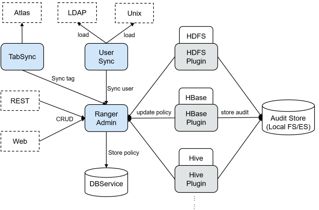
Figure 1-82 Ranger structure
