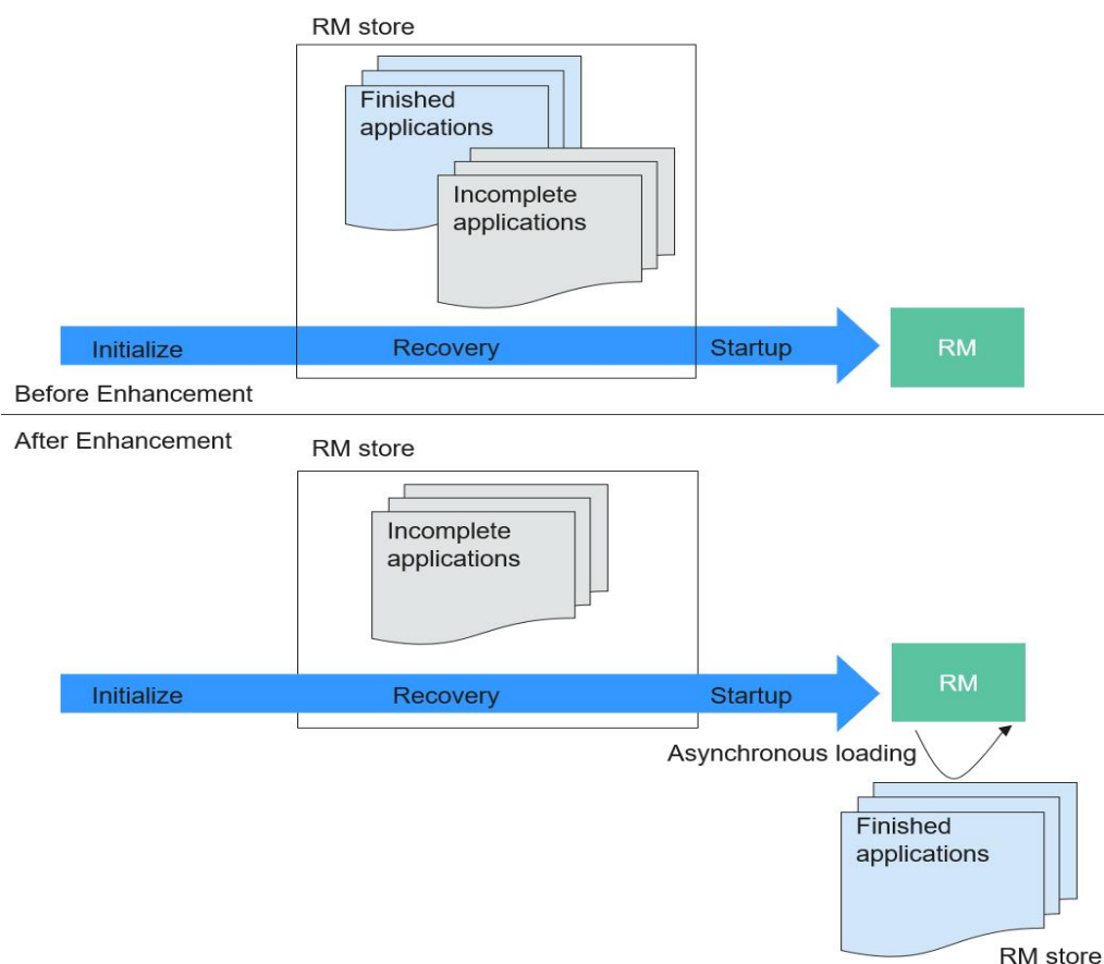
Figure 1-137 Starting the ResourceManager recovery
