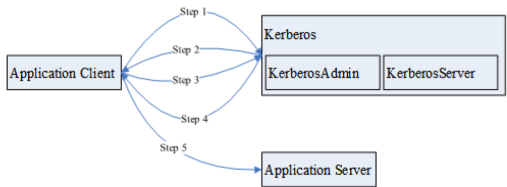
Figure 13-1 Kerberos architecture
