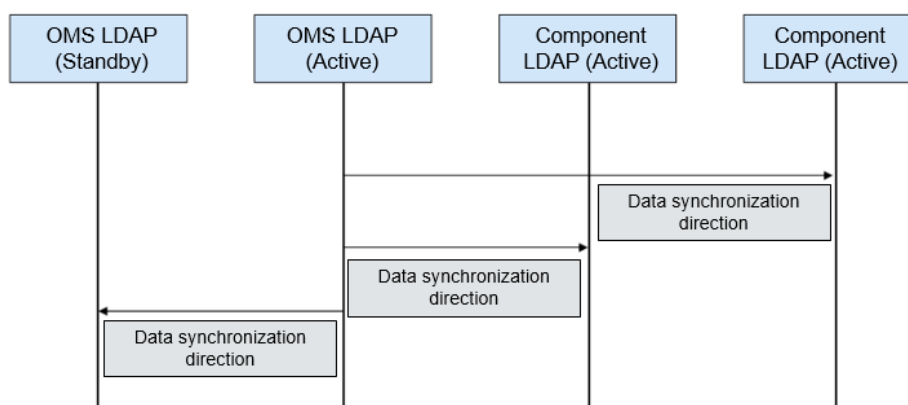
Figure 1-71 LDAP data synchronization
