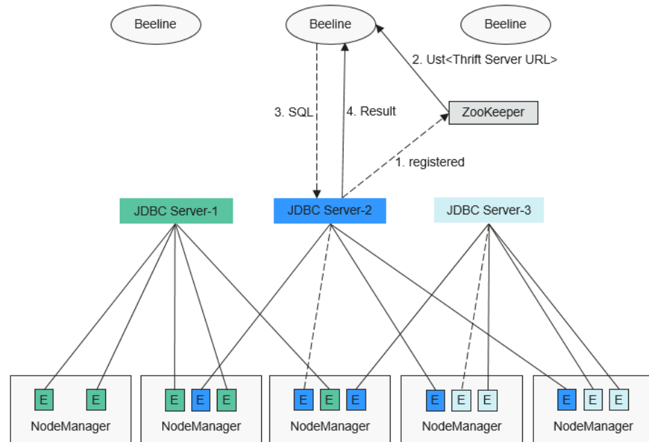
Figure 1-96 Spark JDBCServer HA
