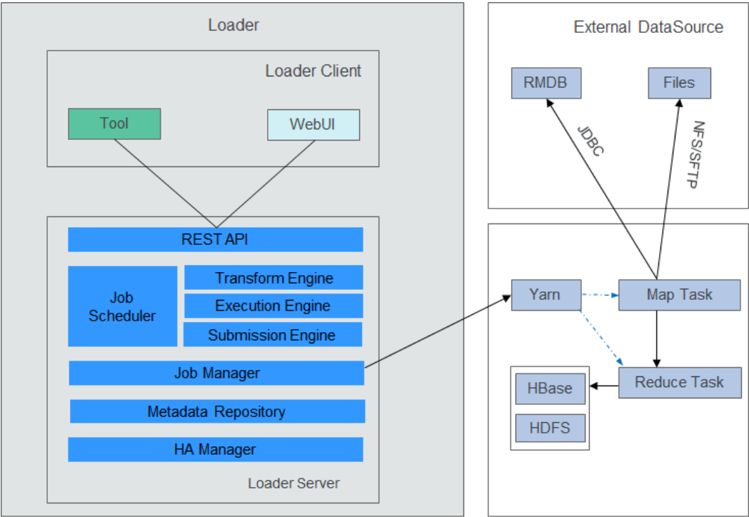
Figure 1-72 Loader model
