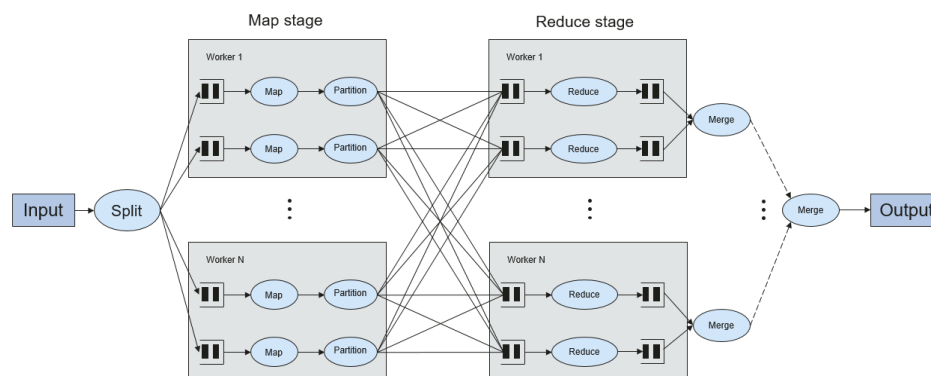
Figure 1-95 Algorithm process
