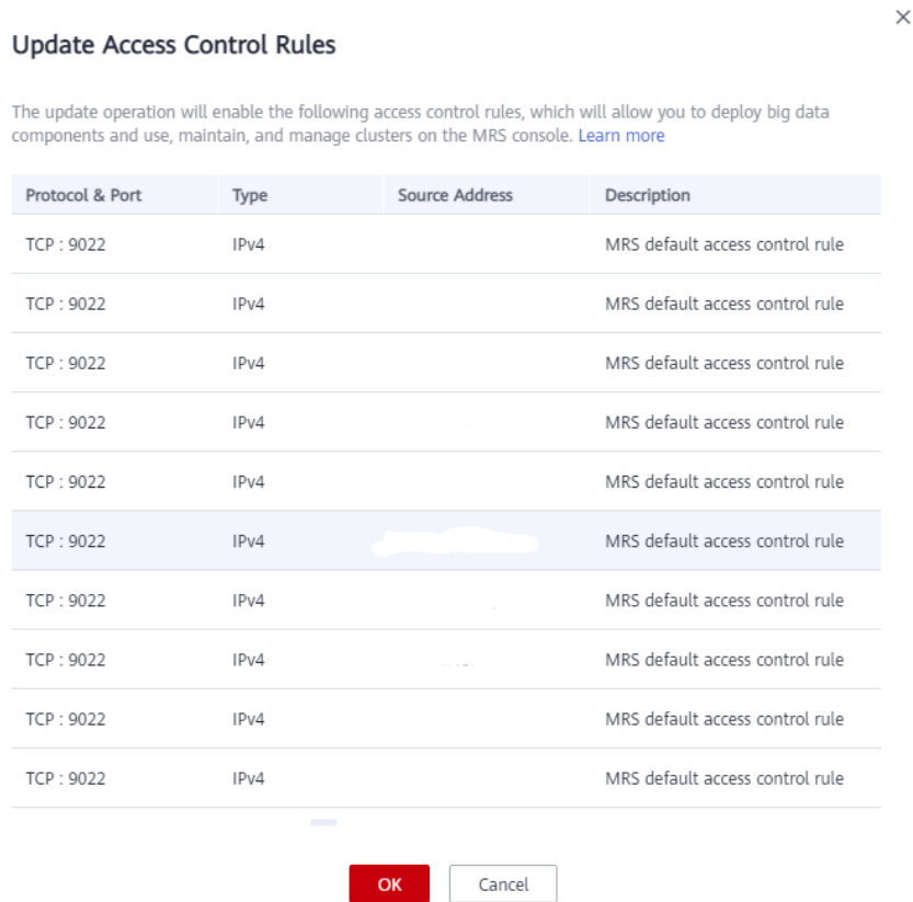
Figure 4-3 Updating access control rules
