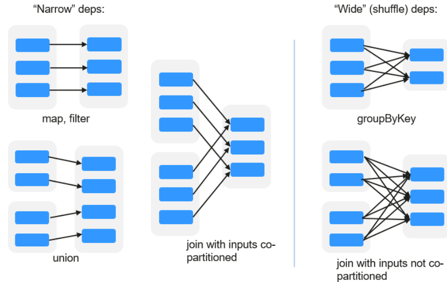
Figure 1-93 RDD dependency
