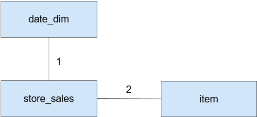
Figure 1-58 Join relationship
