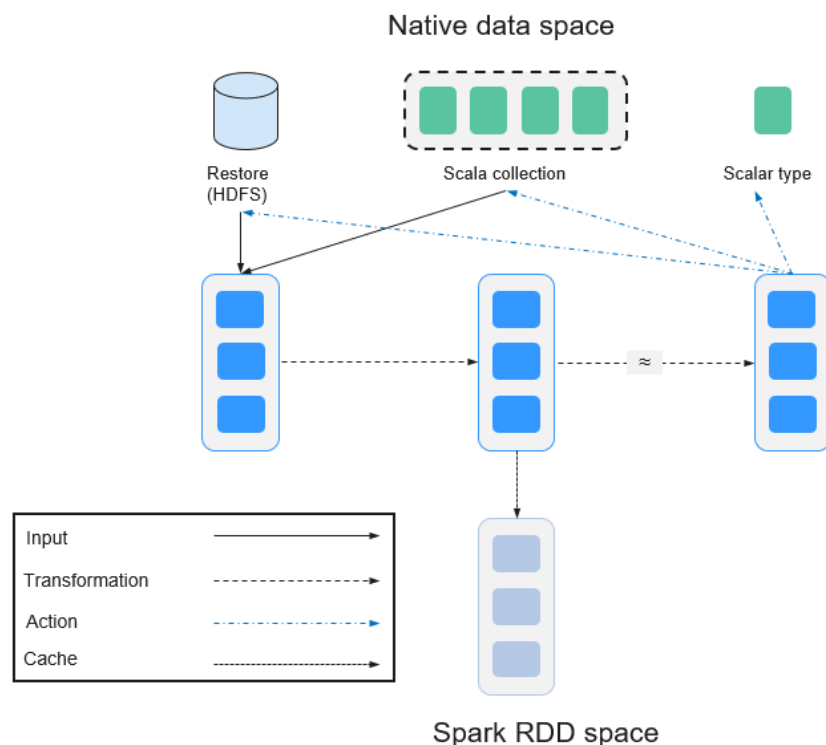
Figure 1-112 RDD operation
