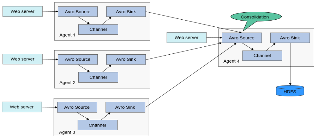
Figure 1-27 Flume cascading
