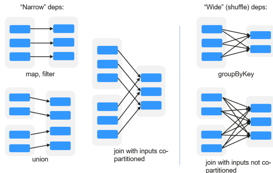
Figure 1-111 RDD dependency
