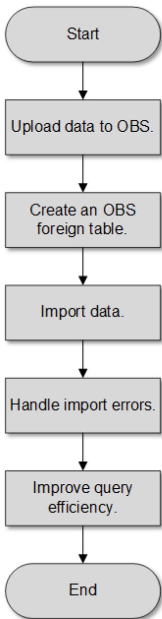
Figure 3-2 Parallel import procedure
