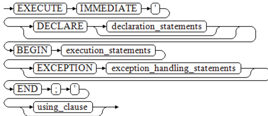
Figure 13-13 call_anonymous_block::=
