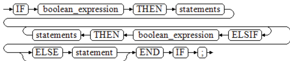
Figure 13-18 IF_THEN_ELSIF_ELSE::=
