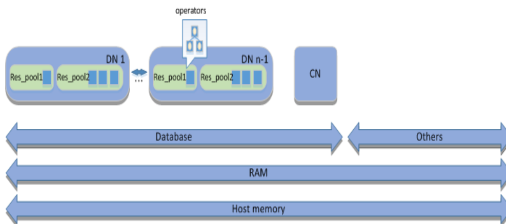
Figure 9-2 Memory usage on a GaussDB(DWS) node
