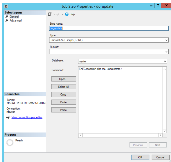
Figure 15-7 Updating statistics
