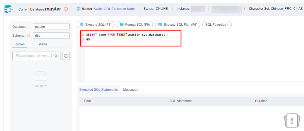
Figure 14-3 Database query
