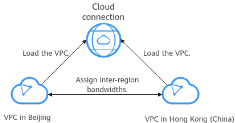
Figure 4-1 Communication between VPCs in different regions
