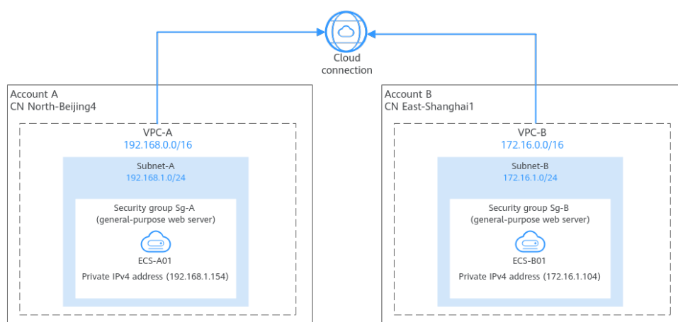
Figure 2-2 Networking planning for connecting VPCs in different regions under different accounts
