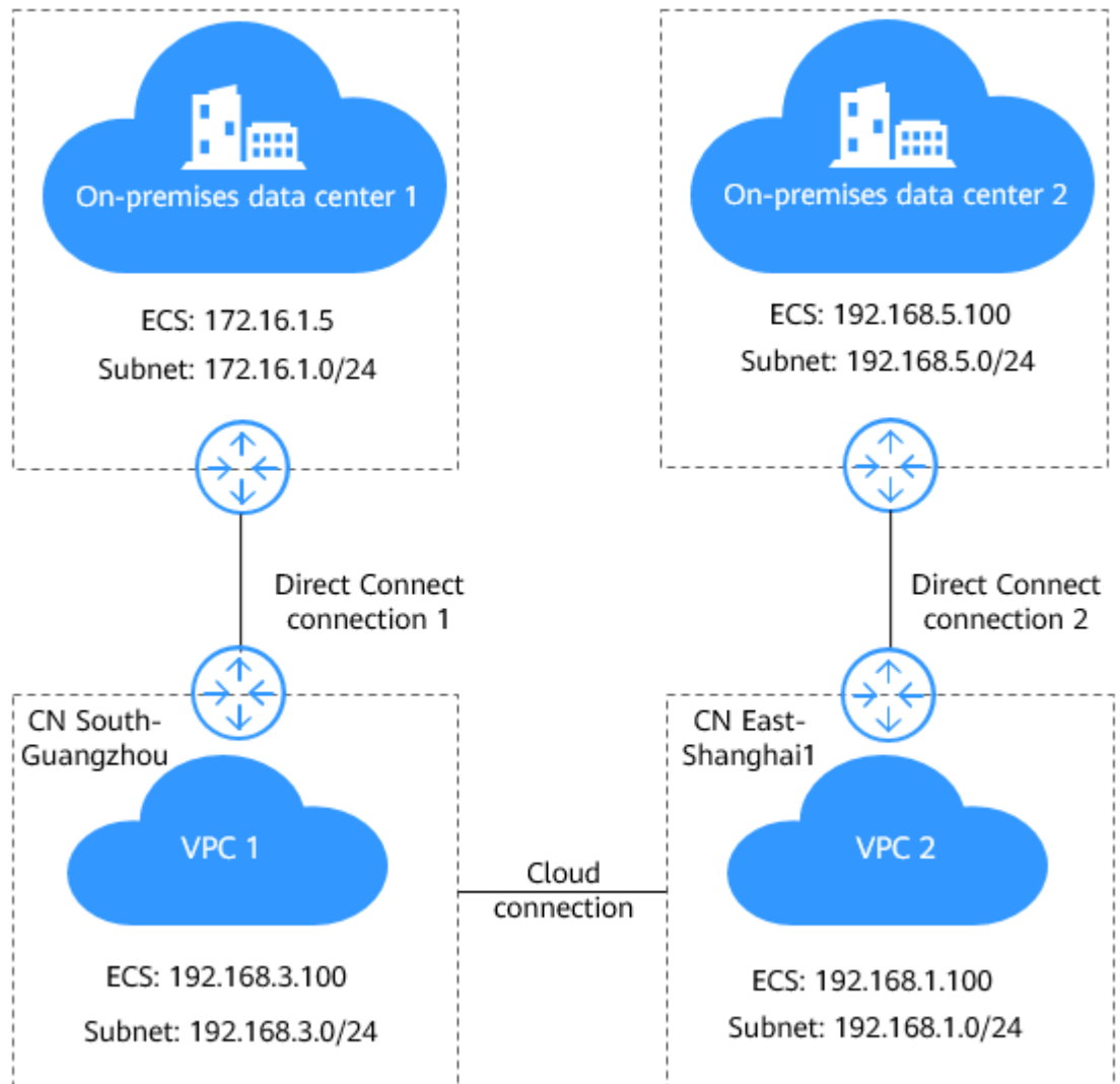
Figure 3-1 Connecting on-premises data centers and VPCs
