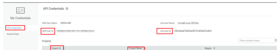
Figure A-2 Obtaining the account ID
