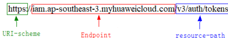
Figure 3-1 Example URI
