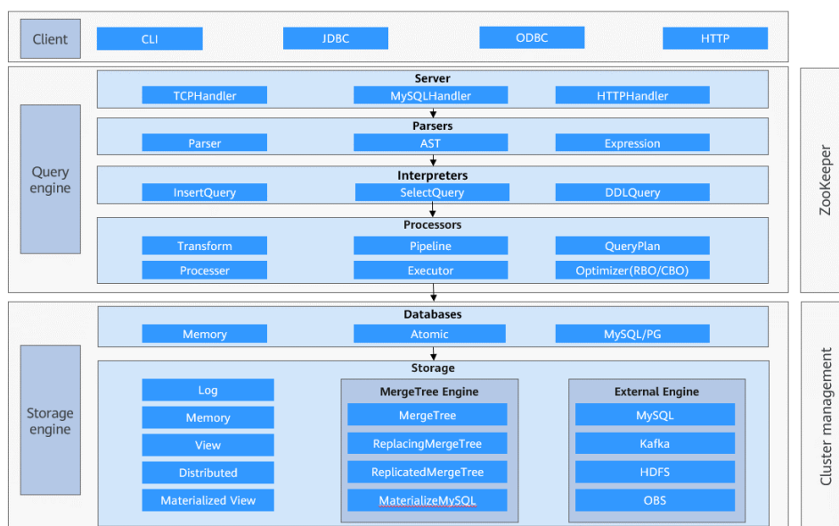
Figure 1-4 ClickHouse architecture
