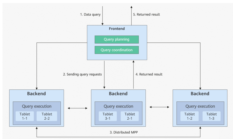
Figure 1-3 Doris architecture
