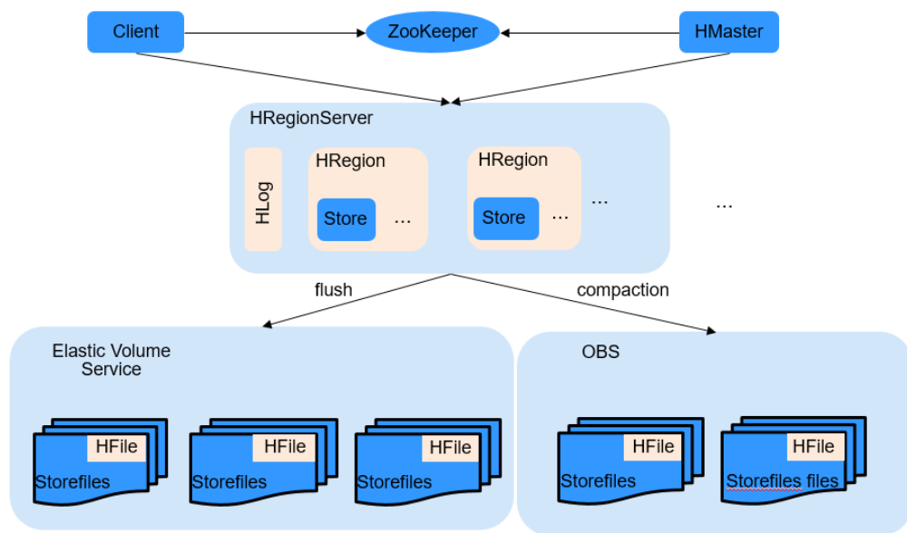
Figure 4-3 Working principles
