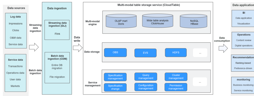
Figure 1-1 Architecture
