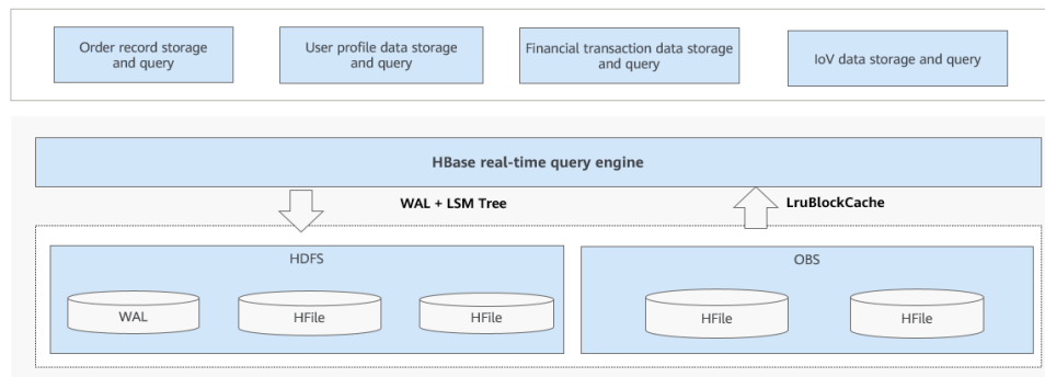
Figure 1-2 HBase architecture
