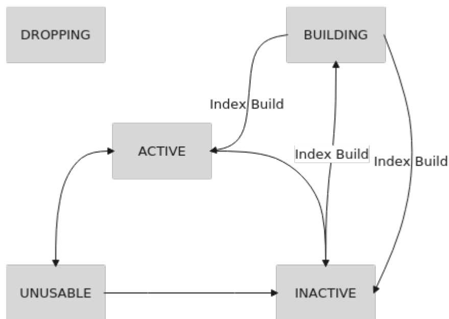
Figure 4-5 State transitions
