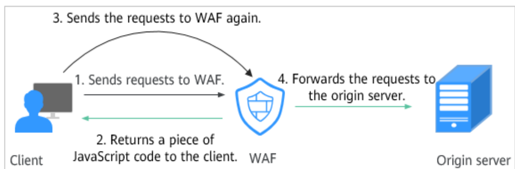
Figure 13-39 JavaScript anti-crawler detection process
