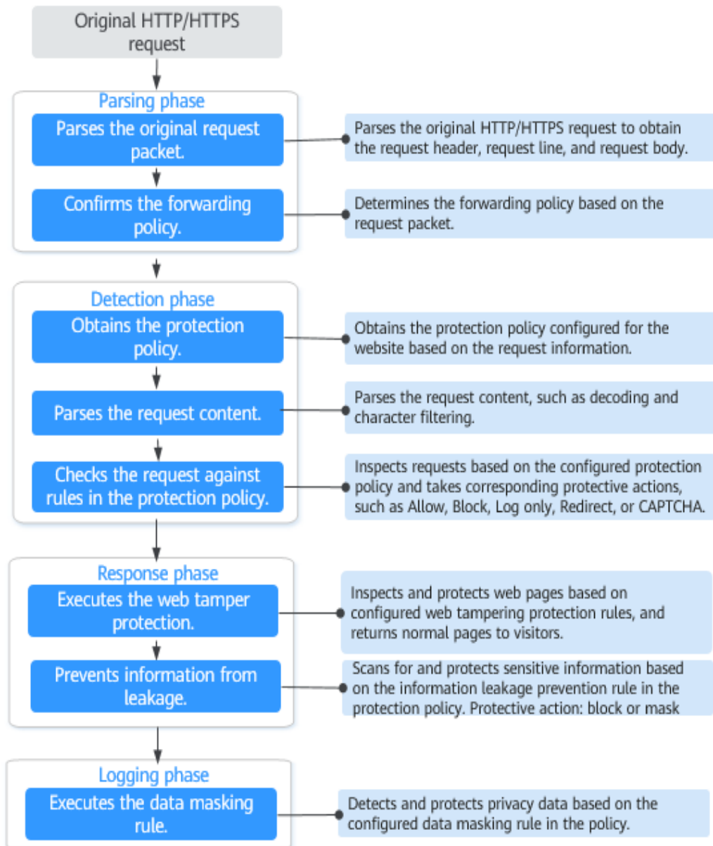
Figure 13-1 WAF engine work process
