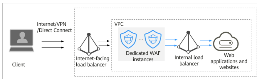
Figure 13-17 Dedicated WAF instance deployment architecture (private network load balancers deployed behind dedicated WAF instances)
