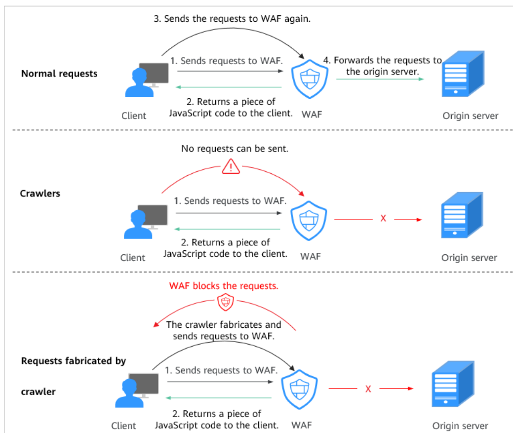
Figure 6-35 JavaScript Anti-Crawler protection process
