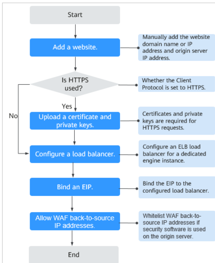
Figure 8-24 Process of connecting a website to a dedicated WAF instance
