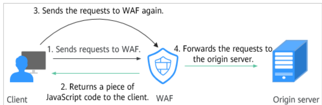
Figure 13-47 JavaScript anti-crawler detection process
