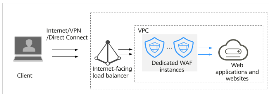
Figure 13-18 Dedicated WAF instance deployment architecture (no private network load balancer deployed behind dedicated WAF instances)
