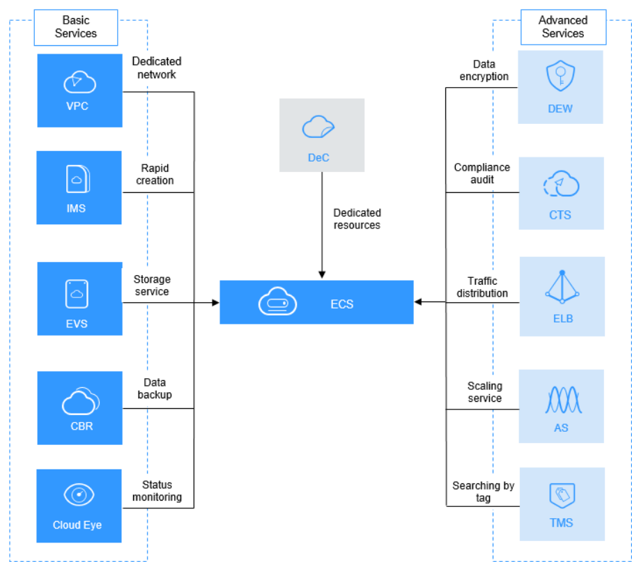
Figure 1-6 Relationships between ECS and other services
