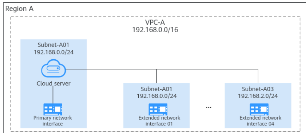
Figure 7-1 Cloud server network interfaces
