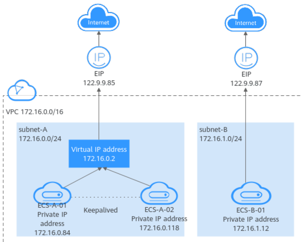
Figure 7-3 Different types of IP addresses used by ECSs
