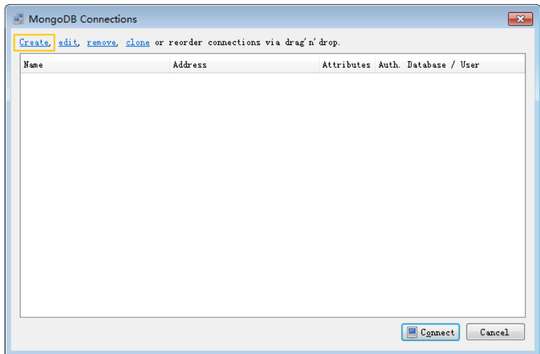
Figure 3-3 Connections
