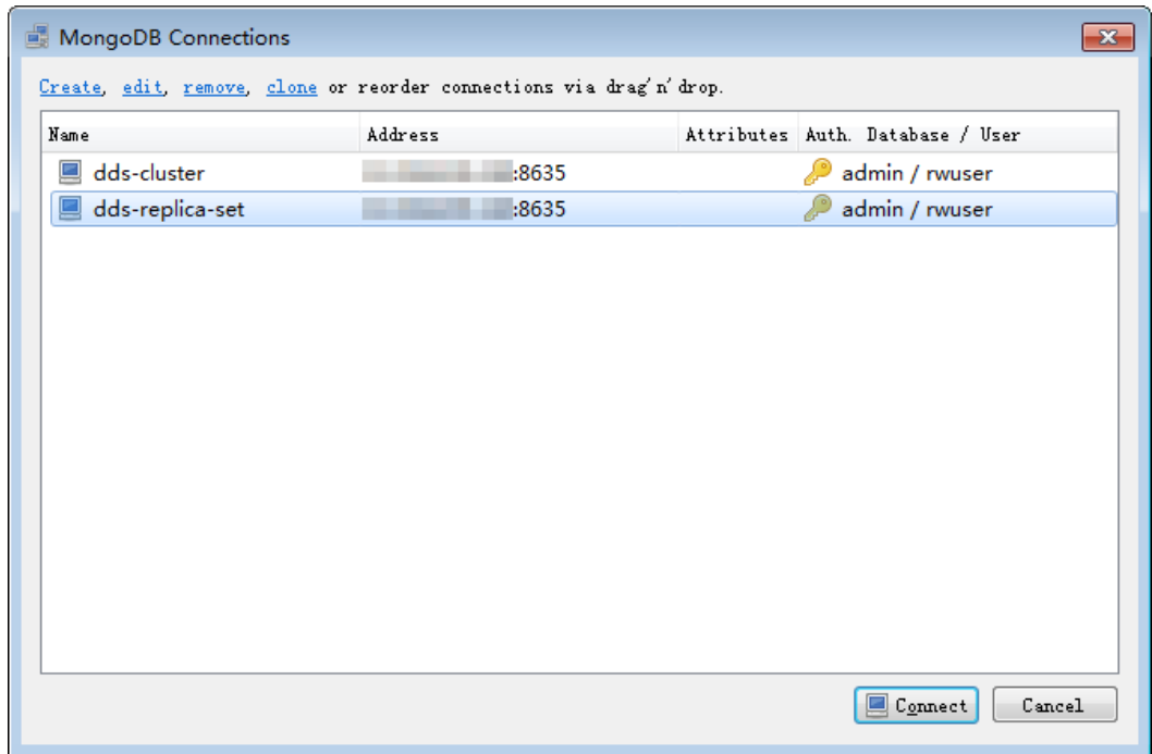
Figure 4-12 Connections
