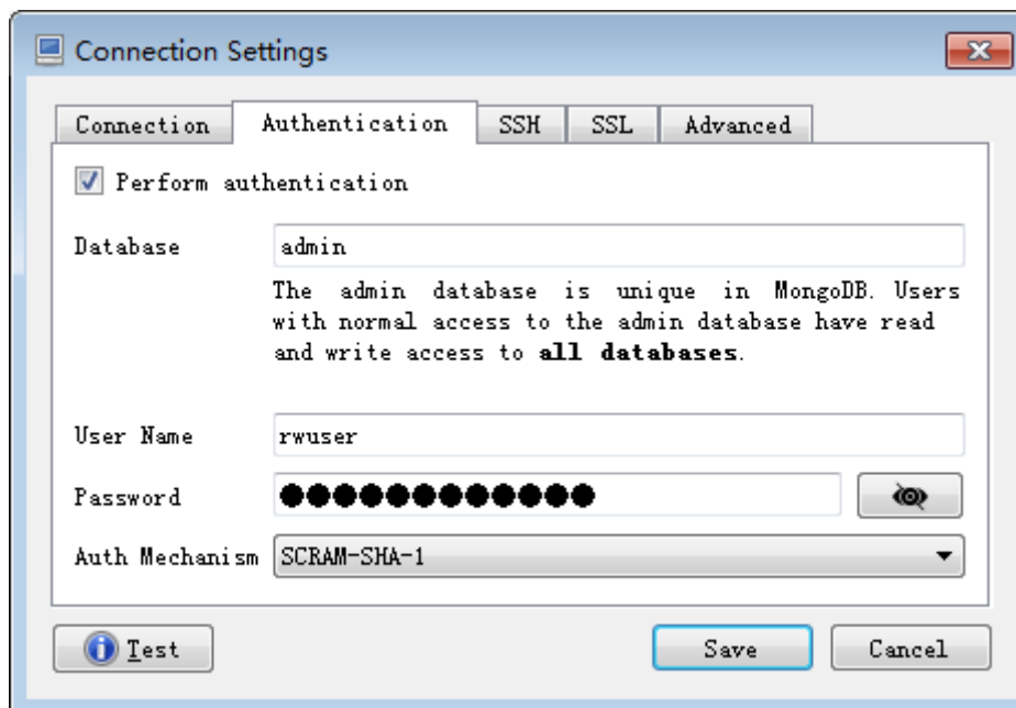
Figure 4-11 Authentication
