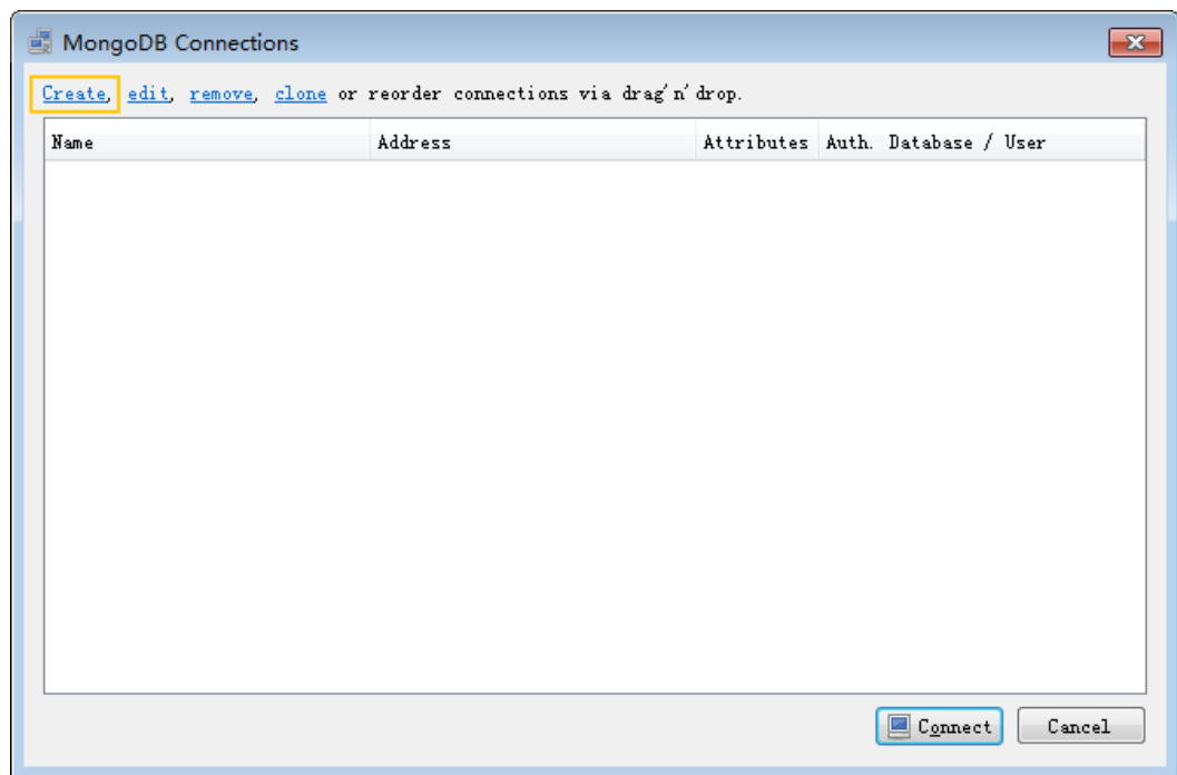
Figure 4-9 Connections
