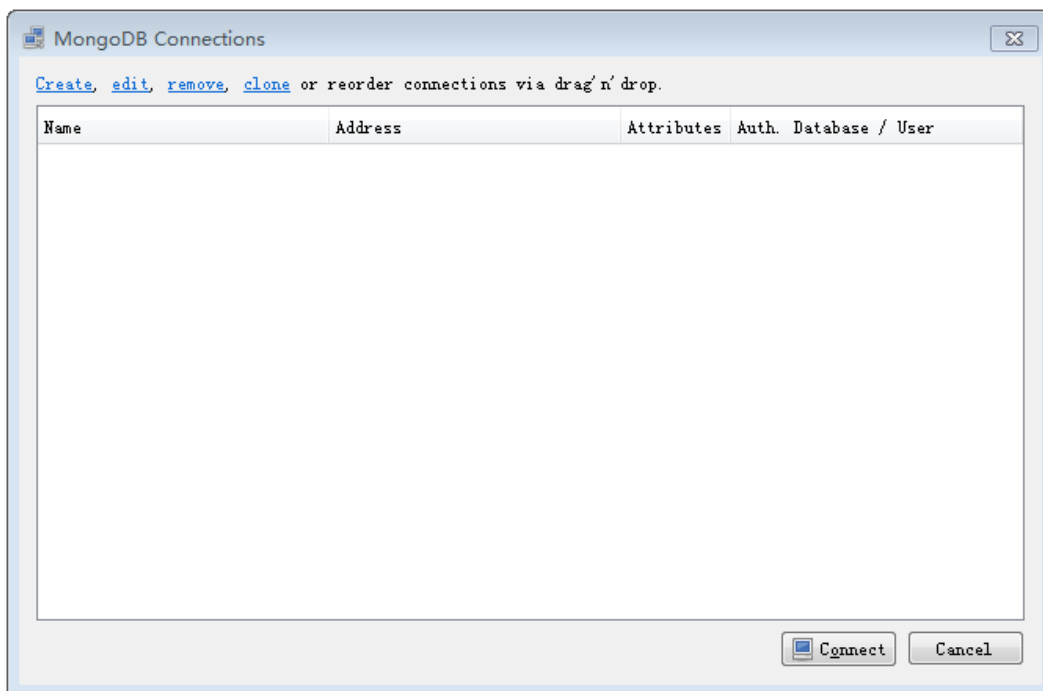
Figure 16-5 Main window
