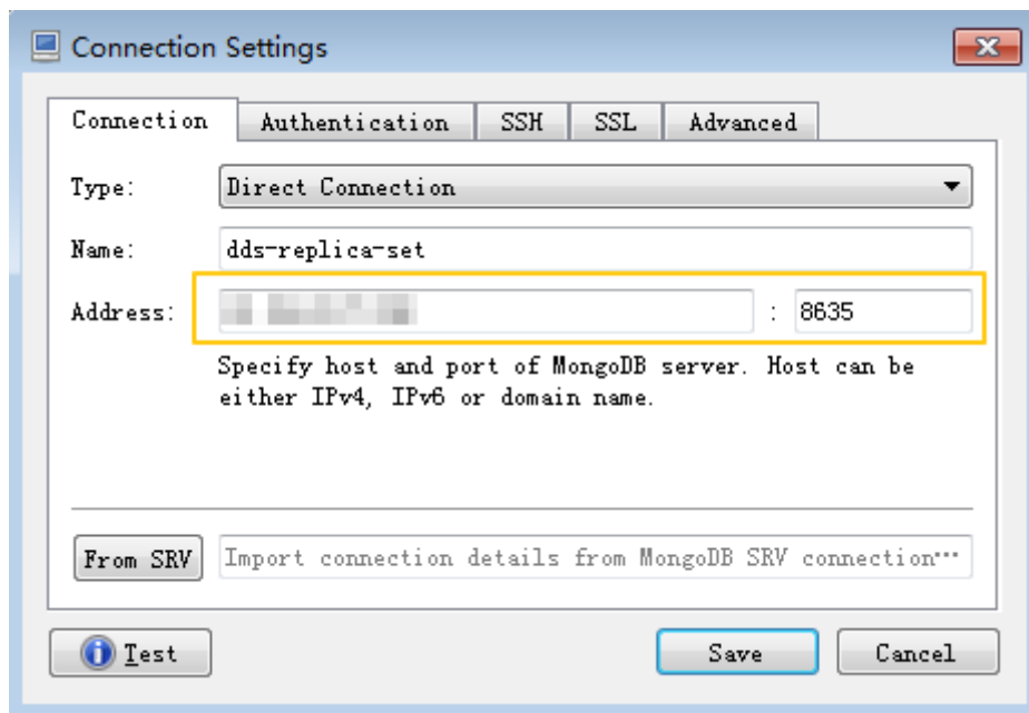
Figure 4-10 Connection
