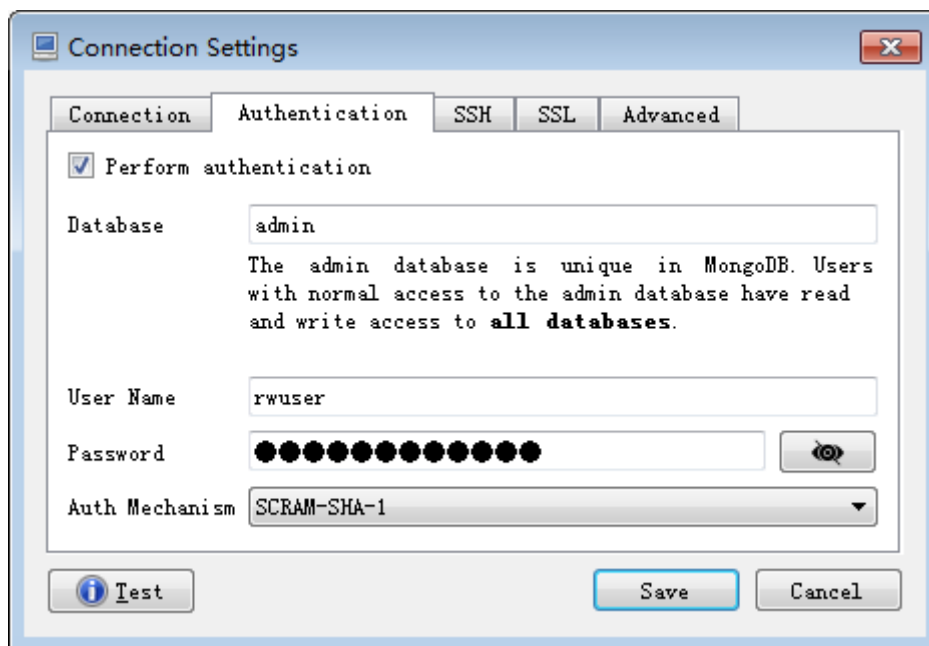
Figure 3-5 Authentication
