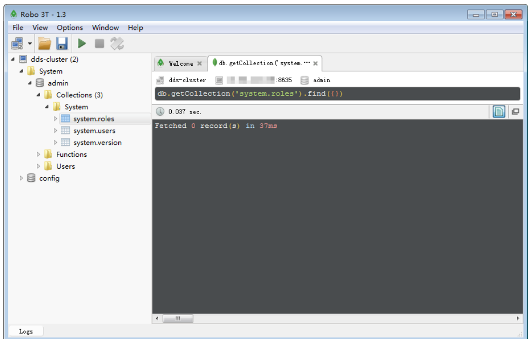
Figure 3-13 Connection succeeded
