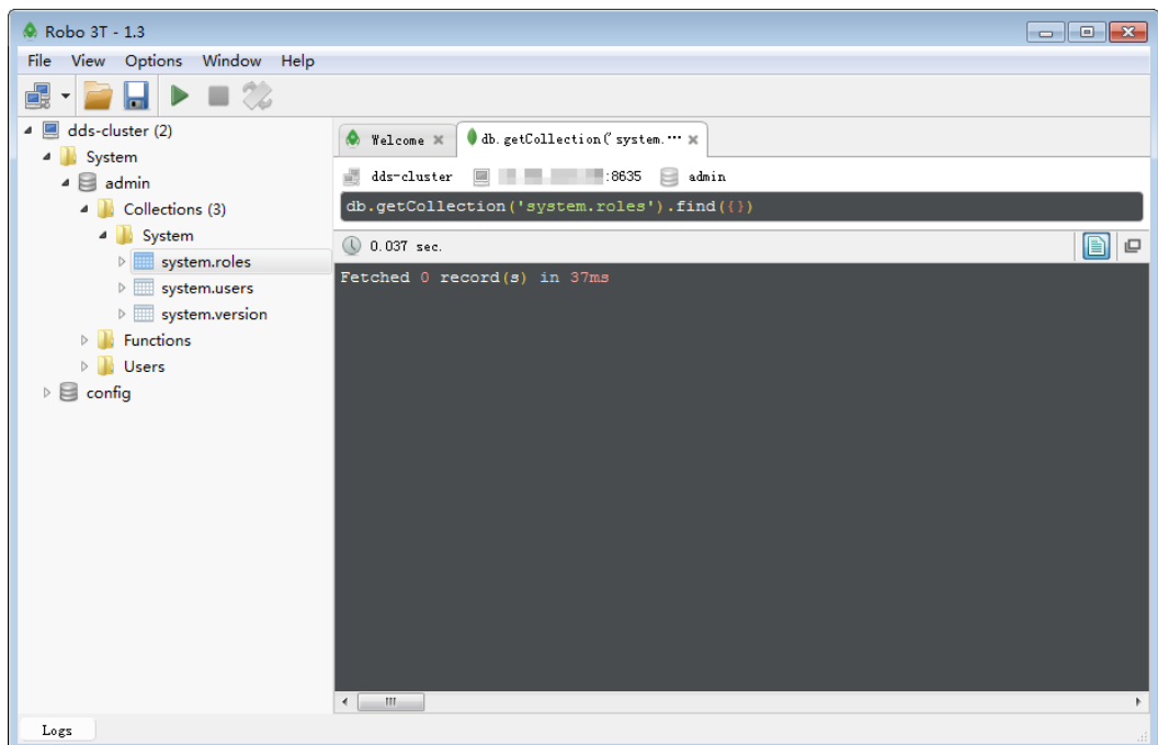
Figure 3-8 Connection succeeded
