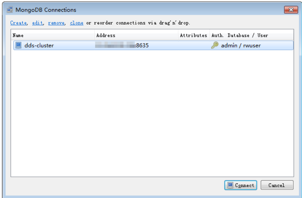
Figure 3-7 Connections
