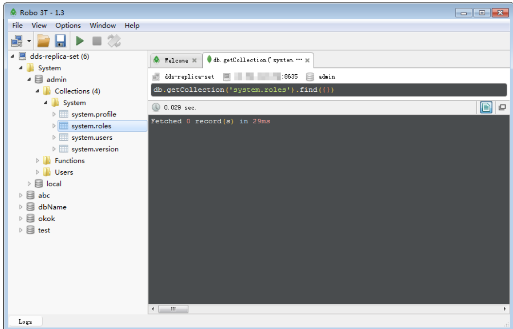
Figure 4-8 Connection succeeded
