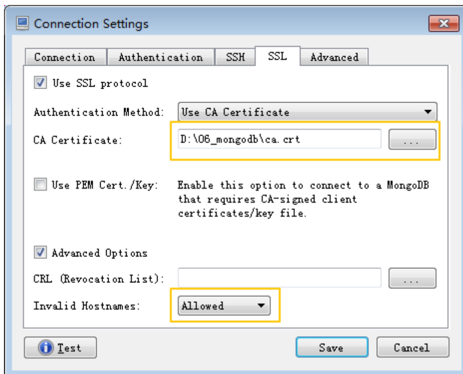
Figure 3-6 SSL
