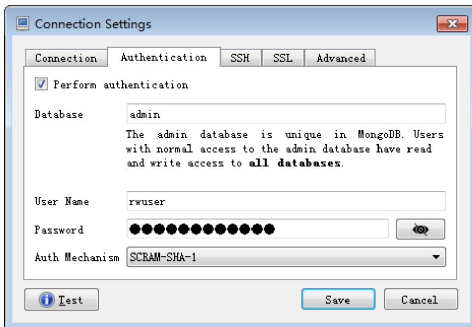
Figure 3-11 Authentication
